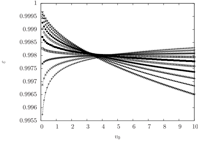
FIG. 3. Coefficient of restitution as a function of the initial relative velocity. Each curve corresponds to a different value of \alpha (from bottom to top on the left side, \alpha varies from 0 to 0.9 in steps of 0.1). The other parameters are: \gamma = 0.001 , m_1 = m_2 = 1 , R_1 = R_2 = 1 , and 2/(5D) = 1 . The lines correspond to the theoretical prediction of Eq. (33).
