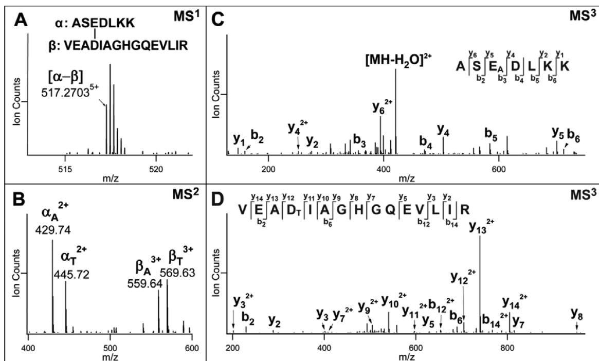
Figure 3. MS n analysis of a representative DHSO interlinked myoglobin peptide. (A) MS spectrum of the interlinked peptide \alpha - \beta ( m/z 517.2703 5+ ). (B) MS 2 spectrum of the interlinked peptide detected in part A. MS 3 spectra of MS 2 fragment ions: (C) \alpha_A ( m/z 429.74 2+ ) and (D) \beta_T ( m/z 569.63 3+ ).
