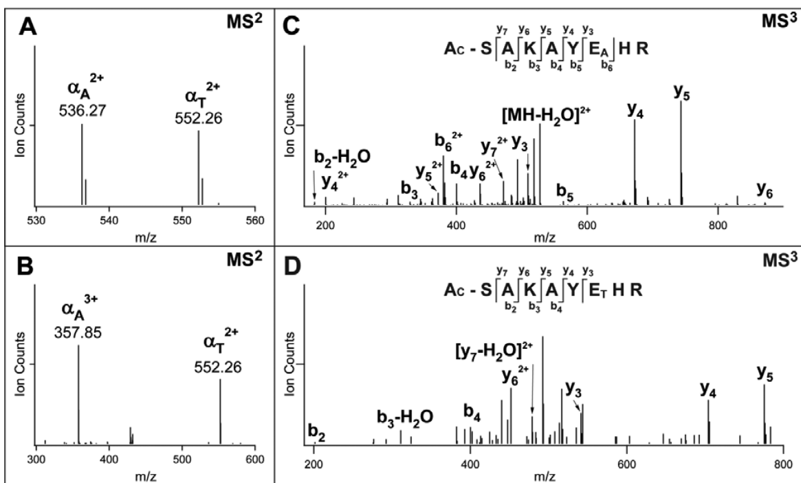
Figure 2. MS n analysis of DHSO interlinked Ac-SR8 homodimer. MS 2 spectra of DHSO interlinked Ac-SR8 at two different charge states: (A) [ \alpha - \alpha ] 4+ ( m/z 548.7623 4+ ) and (B) [ \alpha - \alpha ] 5+ ( m/z 439.2117 5+ ). MS 3 spectra of MS 2 fragment ions detected in part A: (C) \alpha_A ( m/z 536.27 2+ ) and (D) \beta_T ( m/z 552.26 2+ ).
