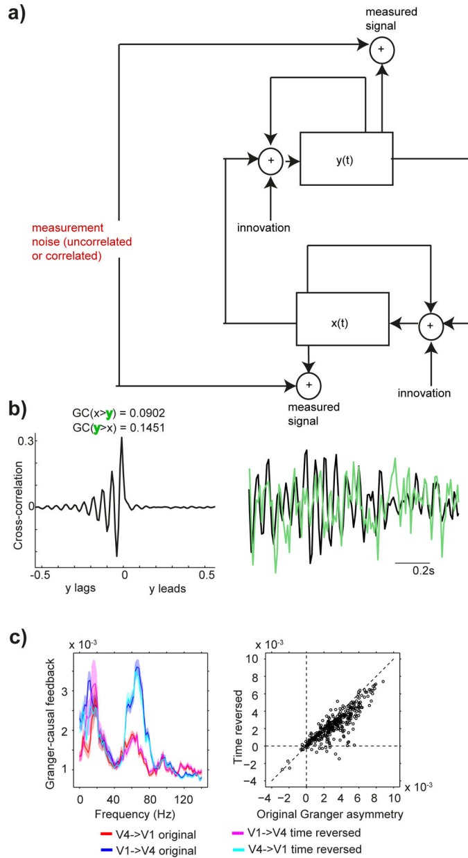
Fig. 5 |. Granger-causal inferences.
