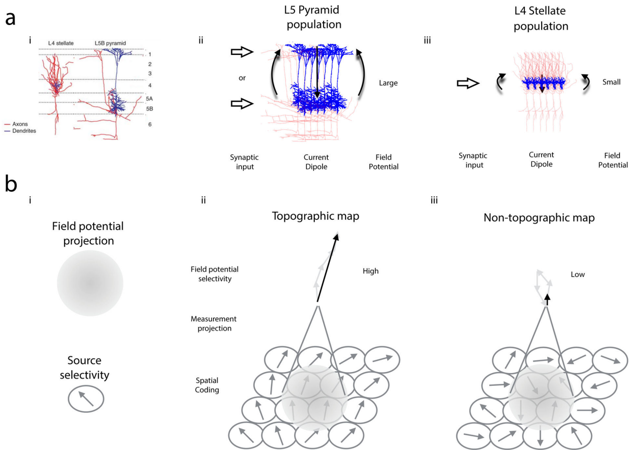
Fig. 2 |. Forward models.
