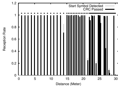
Figure 14: Spatial reception rate profile ( \mathcal{I} high Tx power, SECCED coding)
