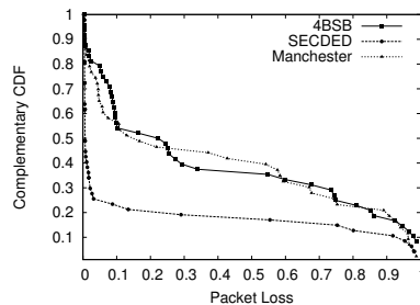
Figure 6: Packet loss v.s. coding schemes in \mathcal{I} , high Tx Power
