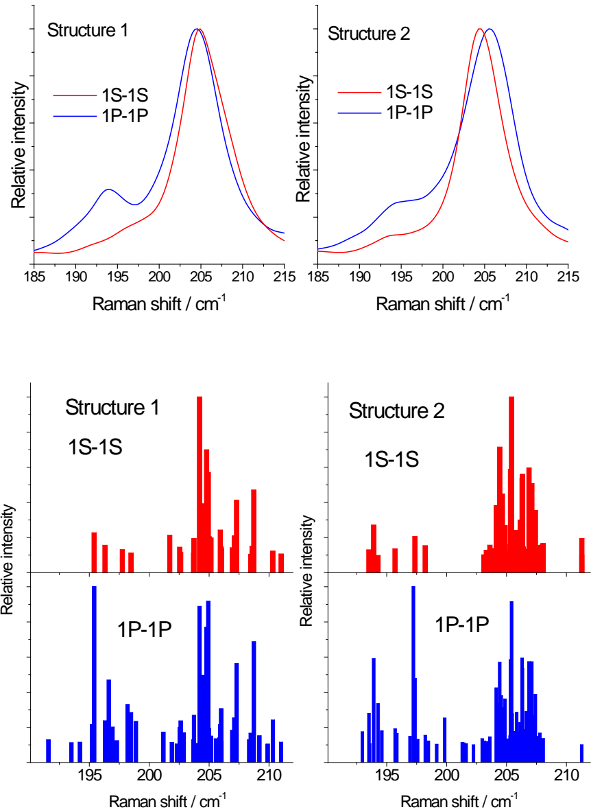
Figure 6. Top: calculated resonance Raman spectra (Tersoff potential) for two separate nanocrystal structures with both 1S_e-1S_{3/2} and 1P_e-1P_{3/2} resonance. Bottom: the individual phonon modes that make up each spectrum. The height of each bar is proportional to its calculated Raman intensity and all modes having at least 10% the intensity of the strongest line are plotted.
