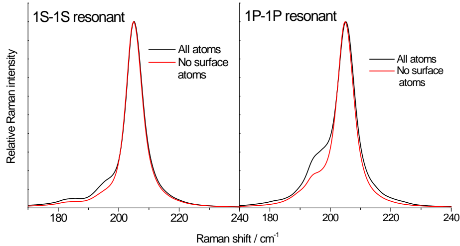
Figure 8. Raman lineshapes (Tersoff potential) for 1S-1S and 1P z -1P z resonant excitation calculated in the usual way (black curves) and calculated assuming that the electron and hole wavefunctions are confined to 75% of the full NC radius (red curves).
