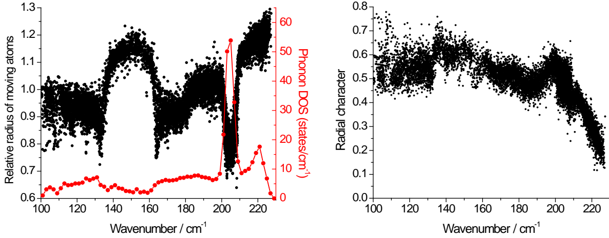
Figure 7. The quantity R_i (eq. 2) and density of states versus mode frequency for all of the phonon modes in the 100-230 \text{cm}^{-1} range for all twelve structures (left panel) and the radial character of each of the modes (right panel).
