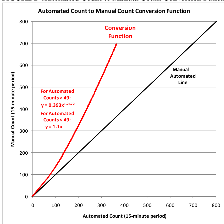
1 FIGURE 2 Automated Count to Manual Count Conversion Function
