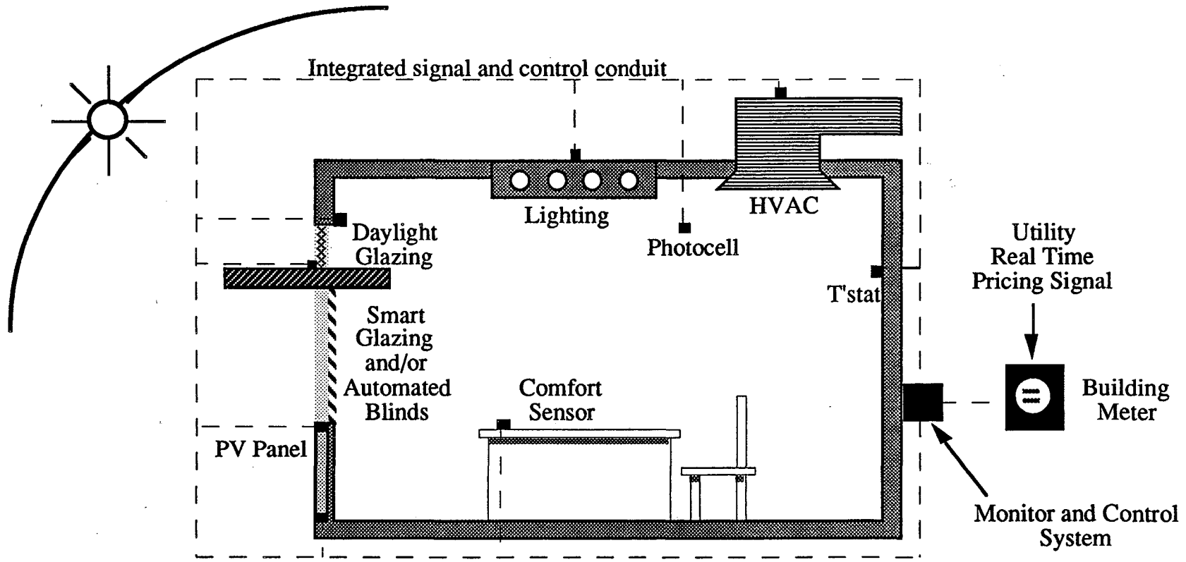
Figure 1. Schematic room section with optimum systems integration. Included here are photovoltaic curtain wall elements (PV), "switchable" glazing, a daylighting optical system (the light shelf), shading devices, and efficient lighting.
