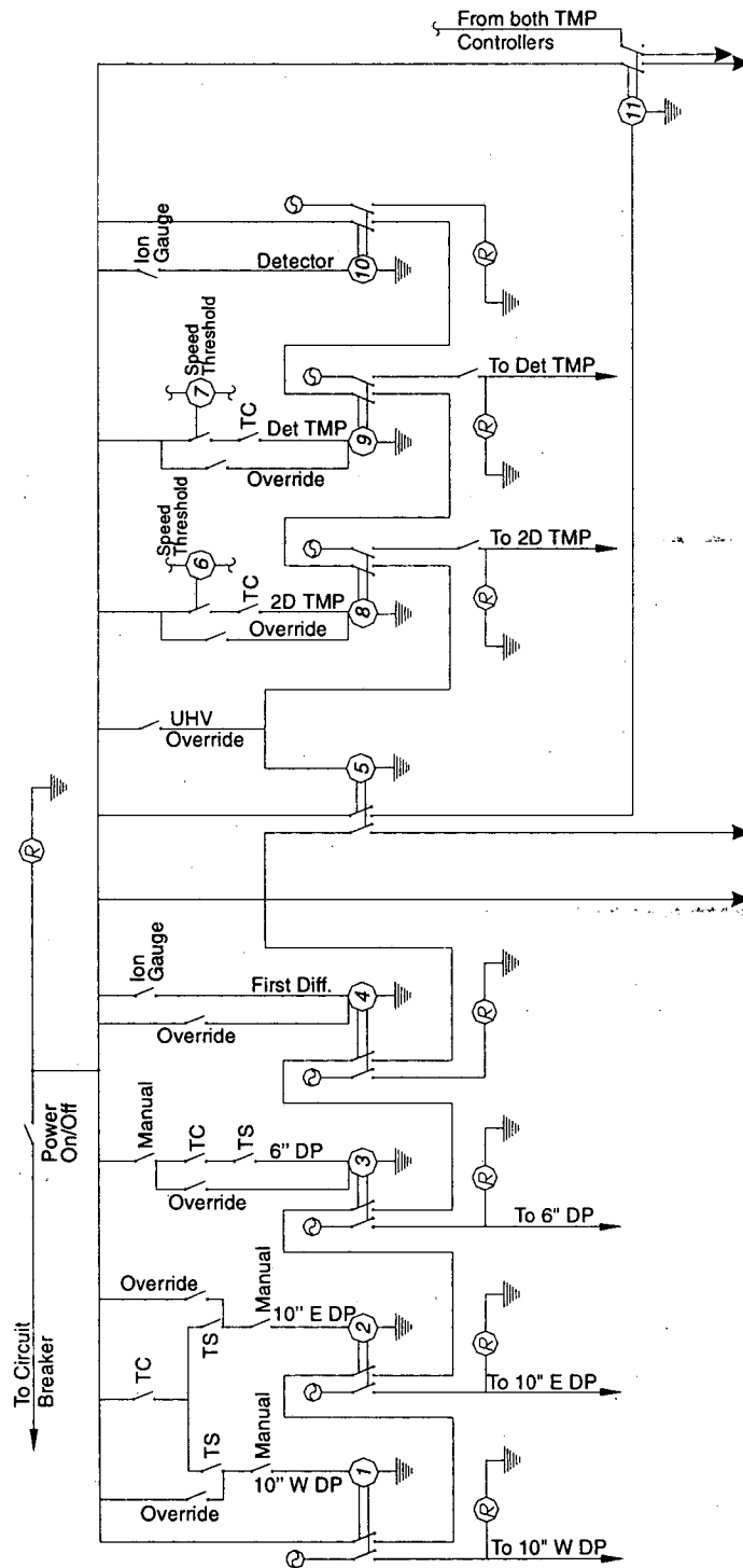
Figure 2a. Interlock box circuit diagram
