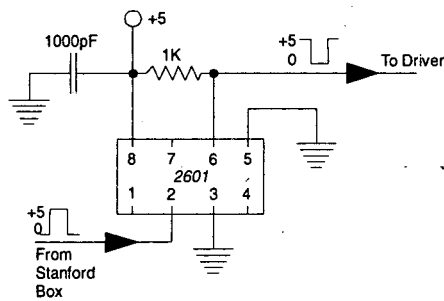
Figure 6.2 Safety optoisolator
