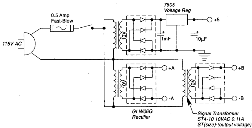
Figure 6.3 Three homemade power supplies
