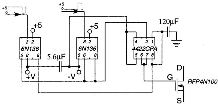
Figure 7.2 Mass gate and decelerator driving circuit
