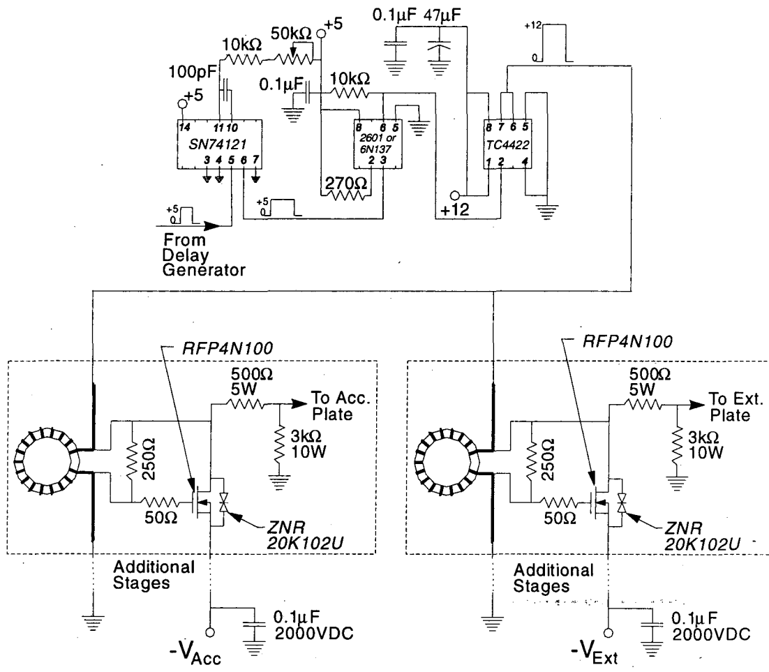
Figure 5.1 Acceleration and extraction circuit diagram
