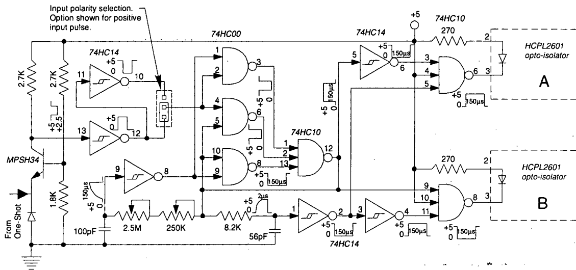
Figure 6.1 Pulsed valve trigger circuit
