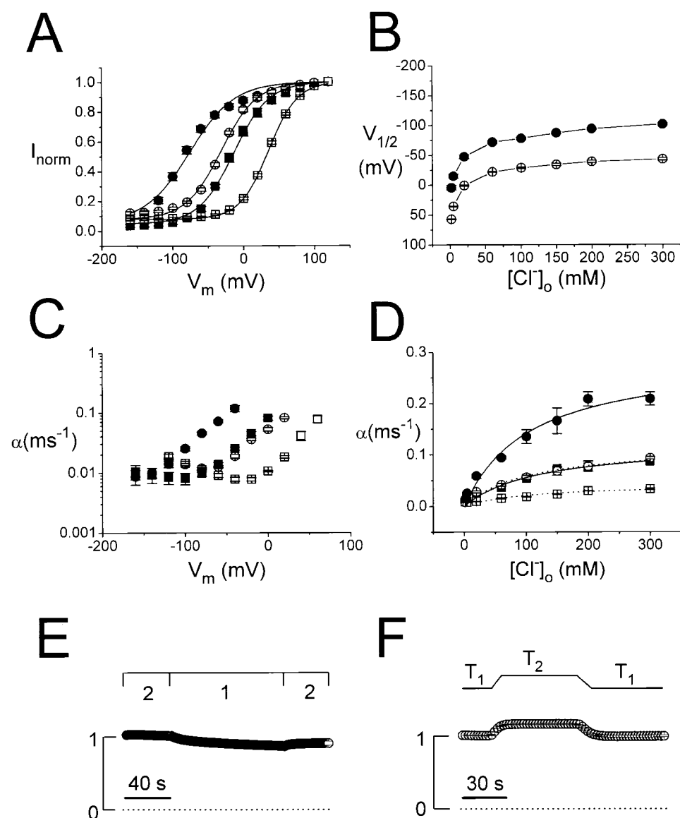
FIGURE 2. Fast- and slow-gating properties of K165 (filled symbols) and K165C* channels (open symbols) derived from macroscopic current recordings. (A) Comparison of the fast-gate P_o - V curves at 100.6 (circles) and 4.6 mM (squares) of [\text{Cl}^-]_o . Solid curves were drawn according to a Boltzmann equation: P_o = P_{\min} + (1 - P_{\min})/[1 + \exp[-zF(V - V_{1/2})/RT]] , with z = 0.8 – 1.2 , P_{\min} = 0.05 – 0.08 . V_{1/2} s in 100.6 and 4.6 mM [\text{Cl}^-]_o were: (K165) -76 and -14 mV; (K165C*) -31 and 35 mV. (B) V_{1/2} s of the fast-gate P_o - V curves as a function of [\text{Cl}^-]_o ( n = 3 – 8 ). (C) Opening rates, \alpha , of the fast gate for K165 and K165C* channels in 100.6 and 4.6 mM [\text{Cl}^-]_o . Symbols are the same as in A ( n = 3 – 8 ). (D) Opening rates of the channels as a function of [\text{Cl}^-]_o . Data points taken at -40 (●) and -80 mV (■) for the K165 channel and at 0 (○) and -40 mV (□) for the K165C* channel. Solid and dotted curves were the best fit to the hyperbolic equation, \alpha = \alpha_{\max}[\text{Cl}^-]_o / (K_{1/2} + [\text{Cl}^-]_o) . The fitted \alpha_{\max} s are ( \text{ms}^{-1} ): K165, 0.29 ( -40 mV) and 0.12 ( -80 mV); K165C*, 0.12 (0 mV) and 0.04 ( -40 mV). The fitted K_{1/2} s are (mM): K165, 107 ( -40 mV) and 121 ( -80 mV); K165C*, 103 (0 mV) and 108 ( -40 mV). (E) Slow-gating transition examined by voltage activation. 30–40 \mu\text{M} MTSEA in the bath solution. Numbers 1 and 2 are the pulsing protocols (see MATERIALS AND METHODS)
