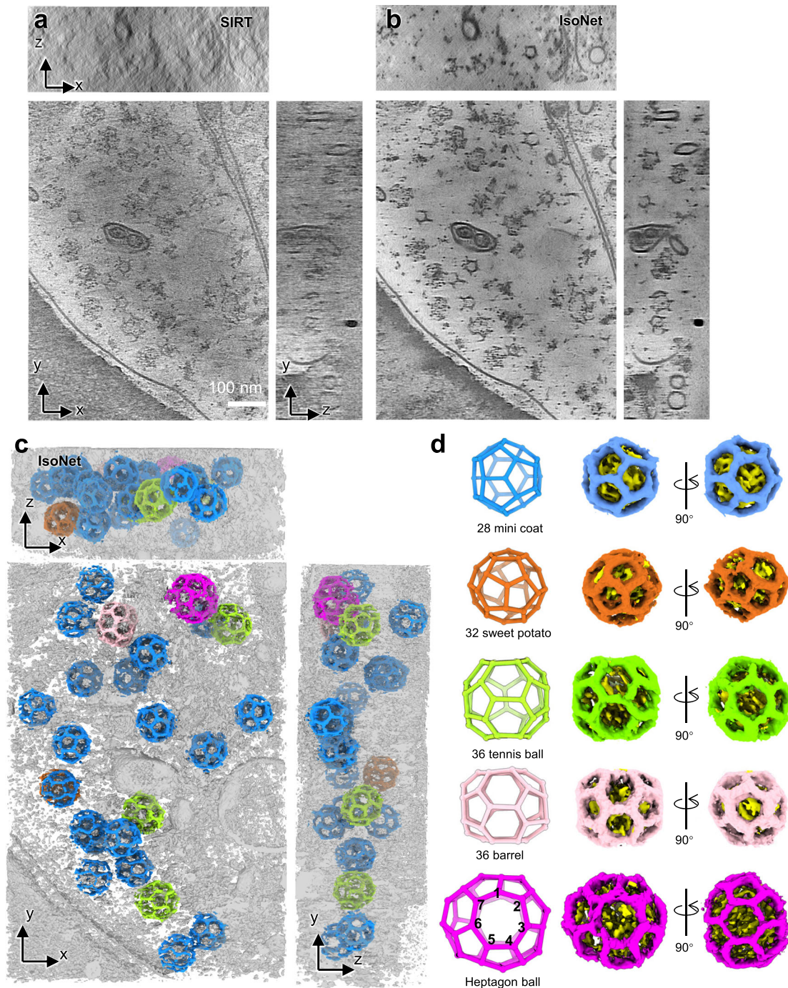
Fig. 6 | IsoNet reveals various types of clathrin cages in a synapse.
