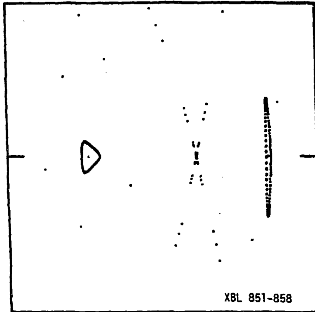
Fig. III.13. T = -0.1100 . De-Vogelaere Variables. Scales: 0.45 to 0.60; \pm 0.003 .
