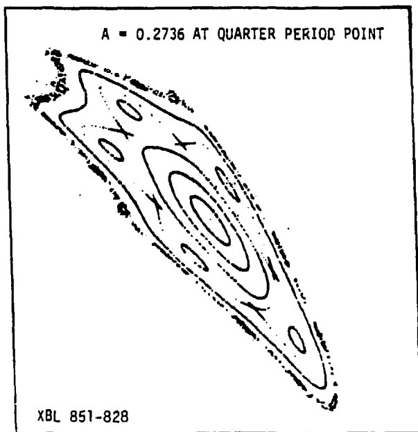
Fig. II.2 Phase plot for the runs of Fig. 1, plotted at Z = \pi/2 \pmod{2\pi} . Scales: Horizontal: -2.0 to 2.0 , for x ; Vertical: -0.6 to 0.6 , for x' .
