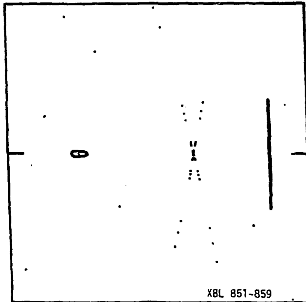
Fig. III.14. T = -0.1125 . De-Vogelaere Variables. Scales: 0.45 to 0.60; \pm 0.003 . Neighborhood of 4th order (unstable) and 8-th order (stable) fixed points just prior to additional bifurcation.
