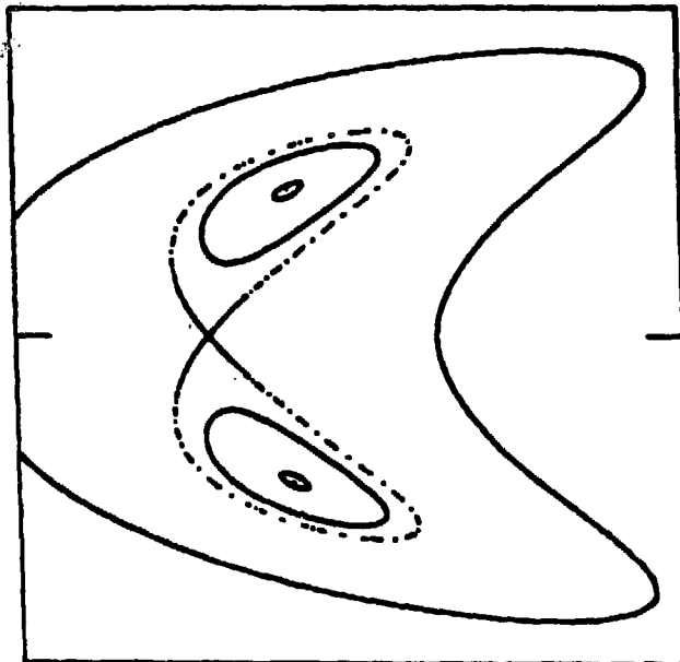
Fig. III.18. T = -0.11223 . De-Vogelaere Variables. Scales: 0.4737 to 0.4738; \pm 0.0001 . After the third bifurcation (leading to Order-32 fixed points), one of the (now unstable) Order-16 fixed points develops vertical loops, that contain stable Order-32 fixed points. The fixed points shown are 4/16: 0.473728930908, 0. 8/32: 0.473741772757, \pm 0.000044371638 . XBL 851-863
