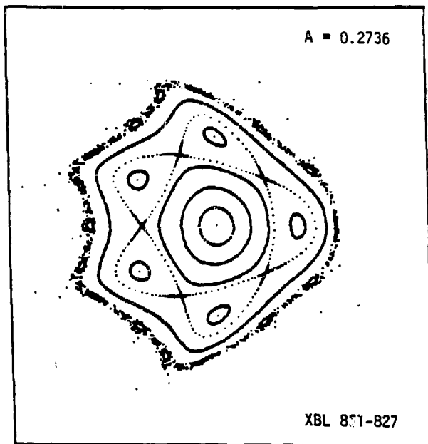
Fig. II.1 x' vs. x phase plot, at Z=0 \pmod{2\pi} , for solutions to Eqn. (1) with A = 0.2736 ( \sigma_0 \approx 74.59 deg.) to the scales:
