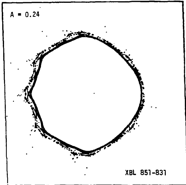
Fig. II.4 Phase Plot for A = 0.24 ; Scales:
