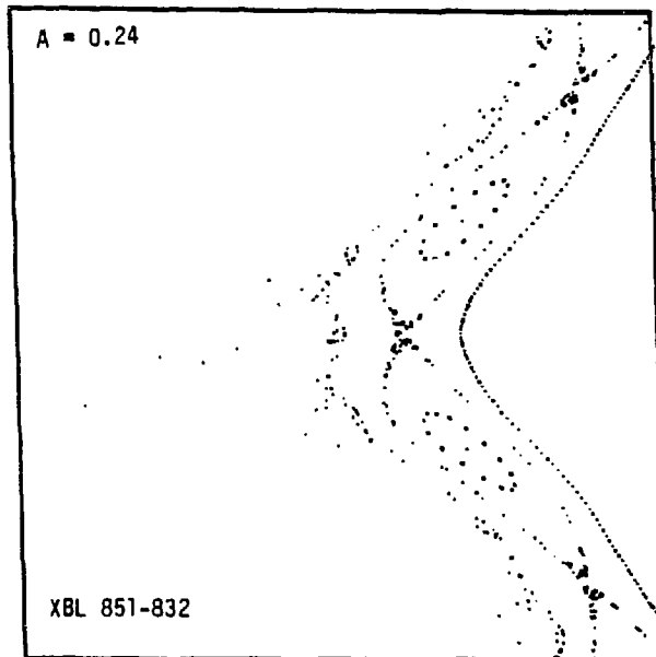
Fig. II.4a Detail related to Fig. II.4 ( A = 0.24 ); Scales:
