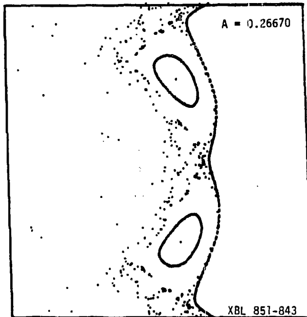
Fig. II.8a Detail related to Fig. II.8 ( A = 0.26670 ); Scales:
