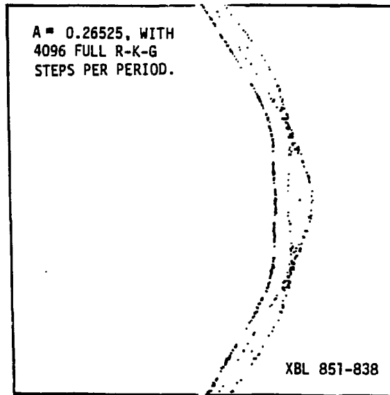
Fig. II.7a Detail related to Fig. II.7 ( A = 0.26525 ); Scales:
