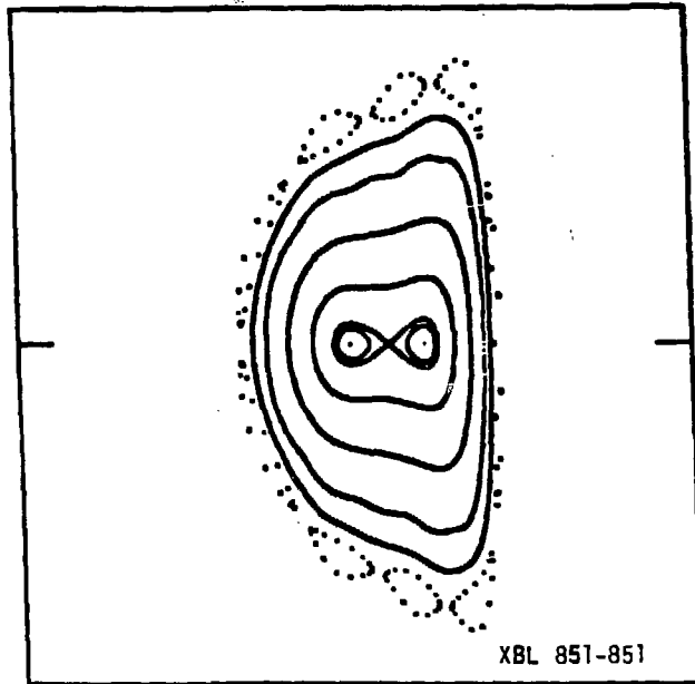
Fig. III.6 T = -0.0136 . De-Vogelaere Variables. Scales: 0.45 to 0.60; \pm 0.003 .
