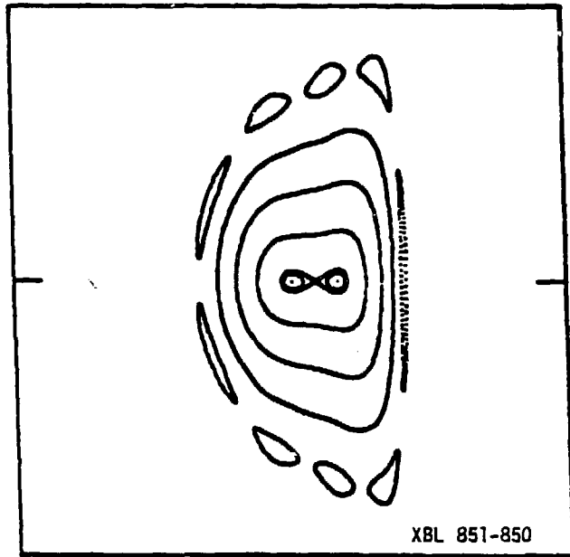
Fig. III.5 T = -0.1035 . De-Vogelaere Variables. Scales: 0.45 to 0.60; \pm 0.003 .
