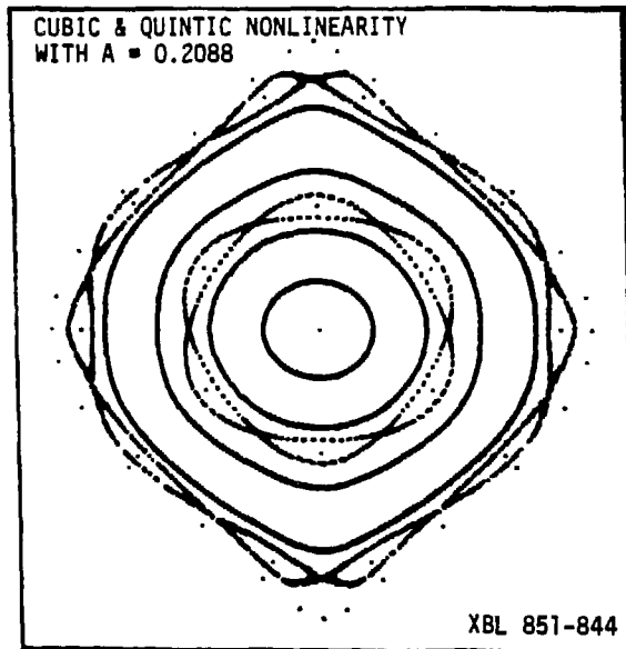
Fig. II.9 Phase plot, at Z = 0 \text{ mod. } 2\pi , for solutions to Eqn. (2) with A = 0.2088 ( \sigma_0 = 55.1621 \text{ deg.} ). Scales:
