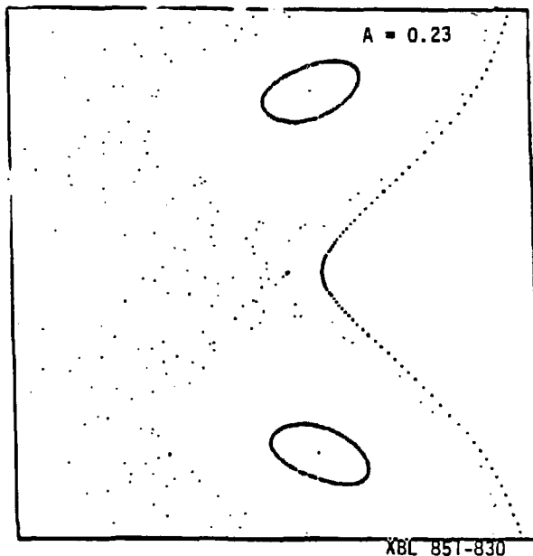
Fig. II.3a Detail related to Fig. II.3 ( A=0.23 ); Scales: Horizontal: -3.0 to -2.0 , for x ; Vertical: -0.08 to 0.08 , for x' . Shown are a portion of the apparently limiting trajectory launched with x_0 = -2.4 , two members of the stable order 7/1 fixed-point system (with surrounding loops), and an unstable sequence of points resulting from a launch substantially at an unstable order 7/1 fixed point.
