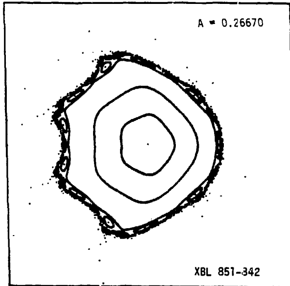
Fig. II.8 Phase plot for A = 0.26670 ; Scales:
