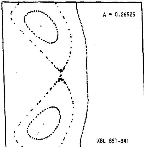
Fig. II.7d Detail related to Fig. II.7 ( A = 0.26525 ); Scales: Horizontal: -2.00 to -1.50 , for x ; Vertical: -0.06 to 0.06 , for x' . Detail of fixed points of order 11/2 systems, indicating possible stochasticity near the unstable order 11/2 fixed point. Also shown is a portion of an apparently smooth phase trajectory of somewhat smaller amplitude that results from a launch with x_0 = -1.7 , x'_0 = 0 .
