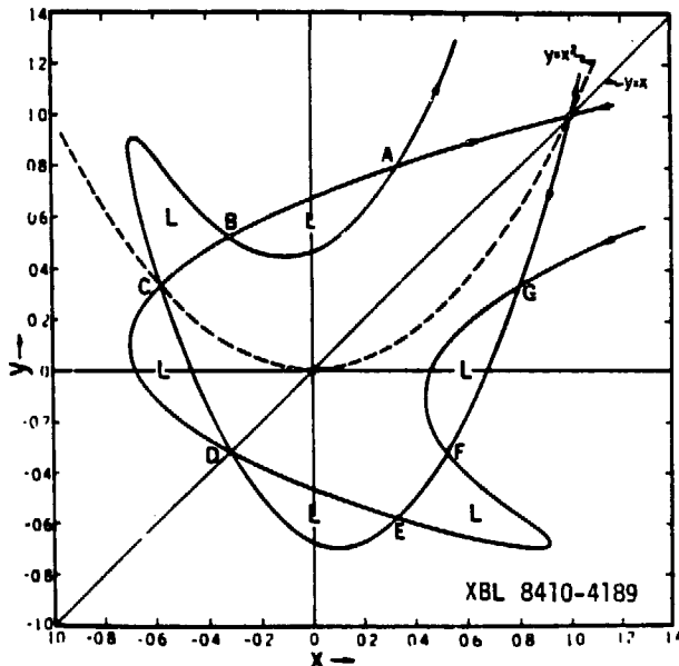
Fig. I.2 Initial portion of trajectories under the transformation x' = y , y' = -x + 2y^2 , leading away from (or toward) the unstable fixed point at x = 1 , y = 1 . The arrows indicate the directions in which points are moved by the transformation. The point pairs AG, BF, CE illustrate the first symmetry, the point pairs AE, BD the second symmetry. The areas of the loops marked L are all equal.
