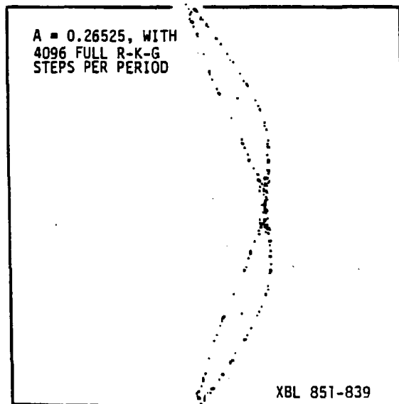
Fig. II.7b Detail related to Fig. II.7 ( A = 0.26525 ); Scales:
