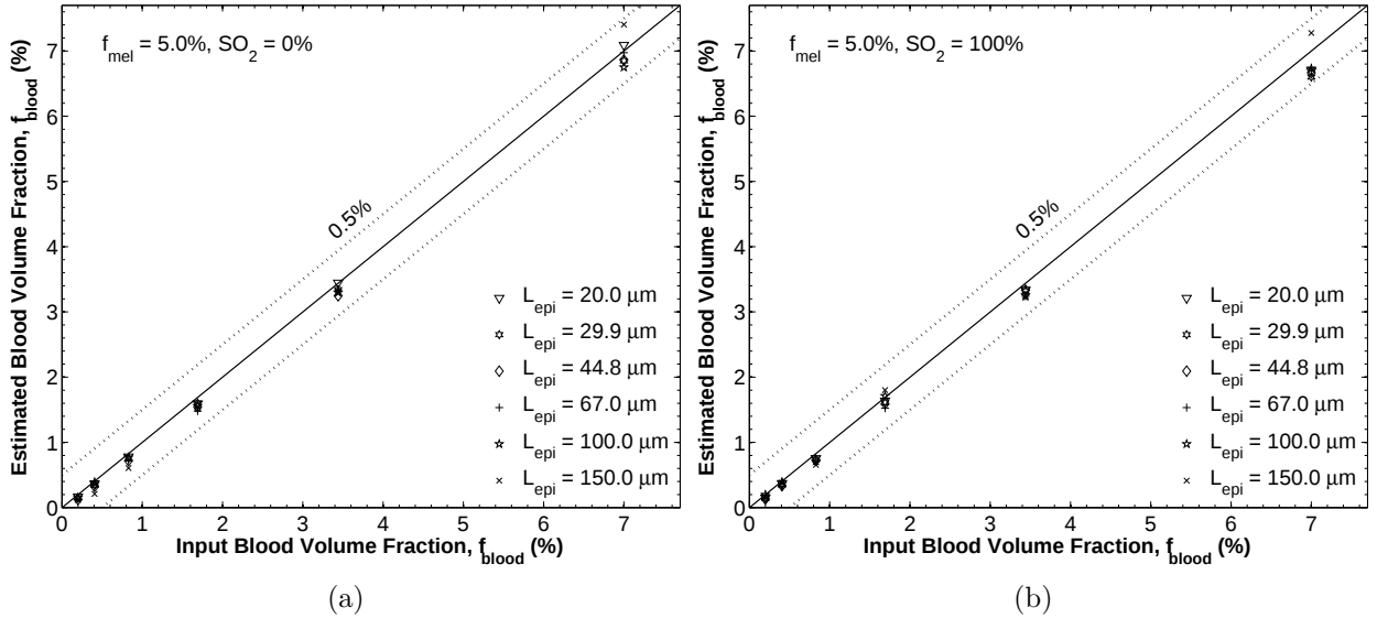
Figure 5: Estimated versus input blood volume fraction f_{blood} and 0.5% absolute error bounds for input values f_{mel} = 5.0\% , 20 \leq L_{epi} \leq 150 \mu m , and (a) SO_2 = 0\% and (b) 100\% , respectively. The scattering constants were taken as C = 5.0 \times 10^5 \text{ cm}^{-1} and b = 1.30 .
