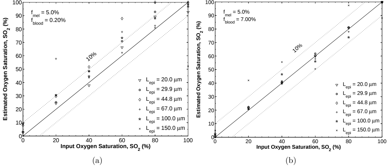
Figure 4: Estimated versus input oxygen saturation SO_2 and 10% absolute error bounds for input values f_{mel} = 5.0\% , 20 \leq L_{epi} \leq 150 \mu\text{m} , and (a) f_{blood} = 0.20\% and (b) 7\% , respectively. The scattering constants were taken as C = 5.0 \times 10^5 \text{ cm}^{-1} and b = 1.30 .
