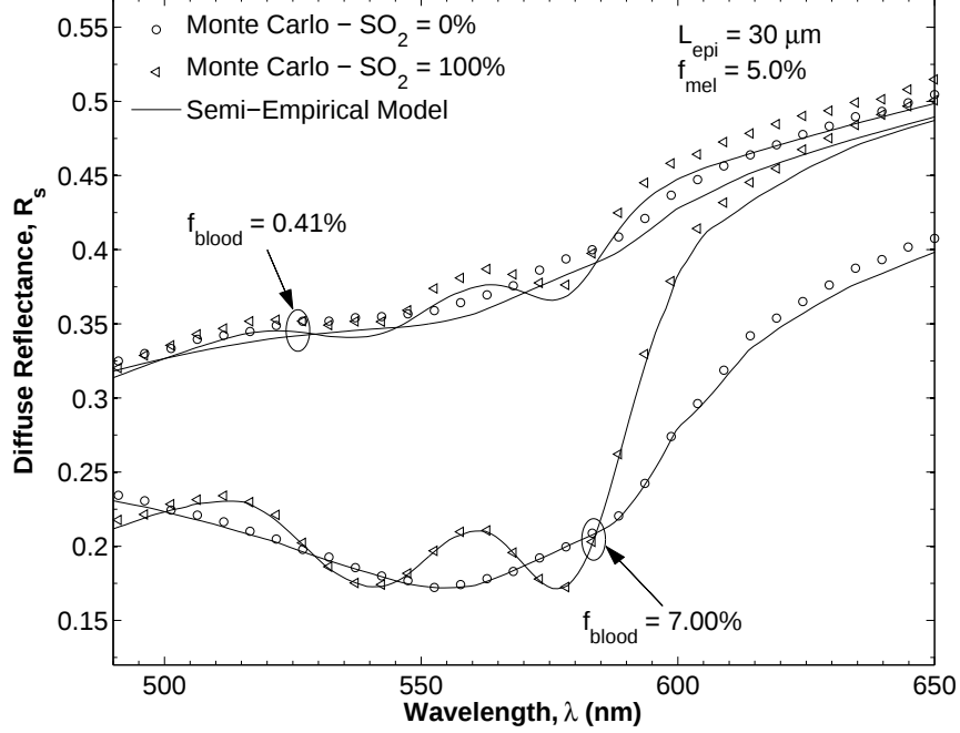
Figure 3: Diffuse reflectance of human skin as a function of wavelength calculated by Monte Carlo simulations and predicted by the semi-empirical model for L_{epi} = 30 \mu\text{m} and f_{mel} = 5.0\% and different values of blood volume fraction f_{blood} (0.41 and 7%) and oxygen saturation SO_2 (0 and 100%).
