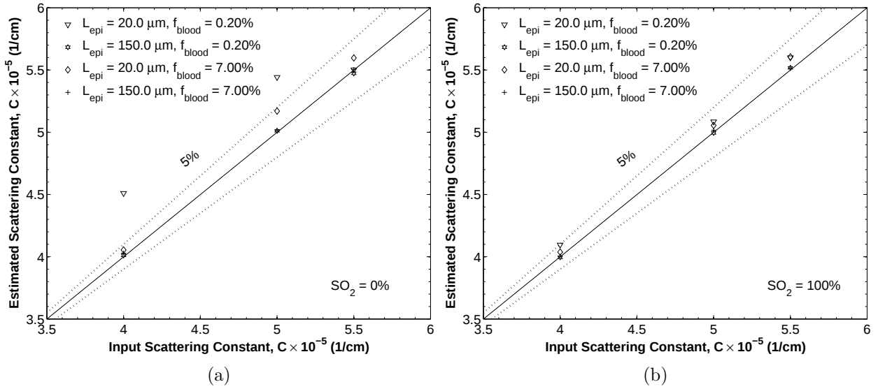
Figure 8: Estimated versus input scattering constant C and 5% relative error bounds for input values 20 \leq L_{epi} \leq 150 \text{ } \mu\text{m} , 0.20 \leq f_{blood} \leq 7.0\% , f_{mel} = 5.0\% , b = 1.30 for (a) SO_2 = 0\% and (b) SO_2 = 100\% , respectively. The scattering constant b is assumed to be known.
