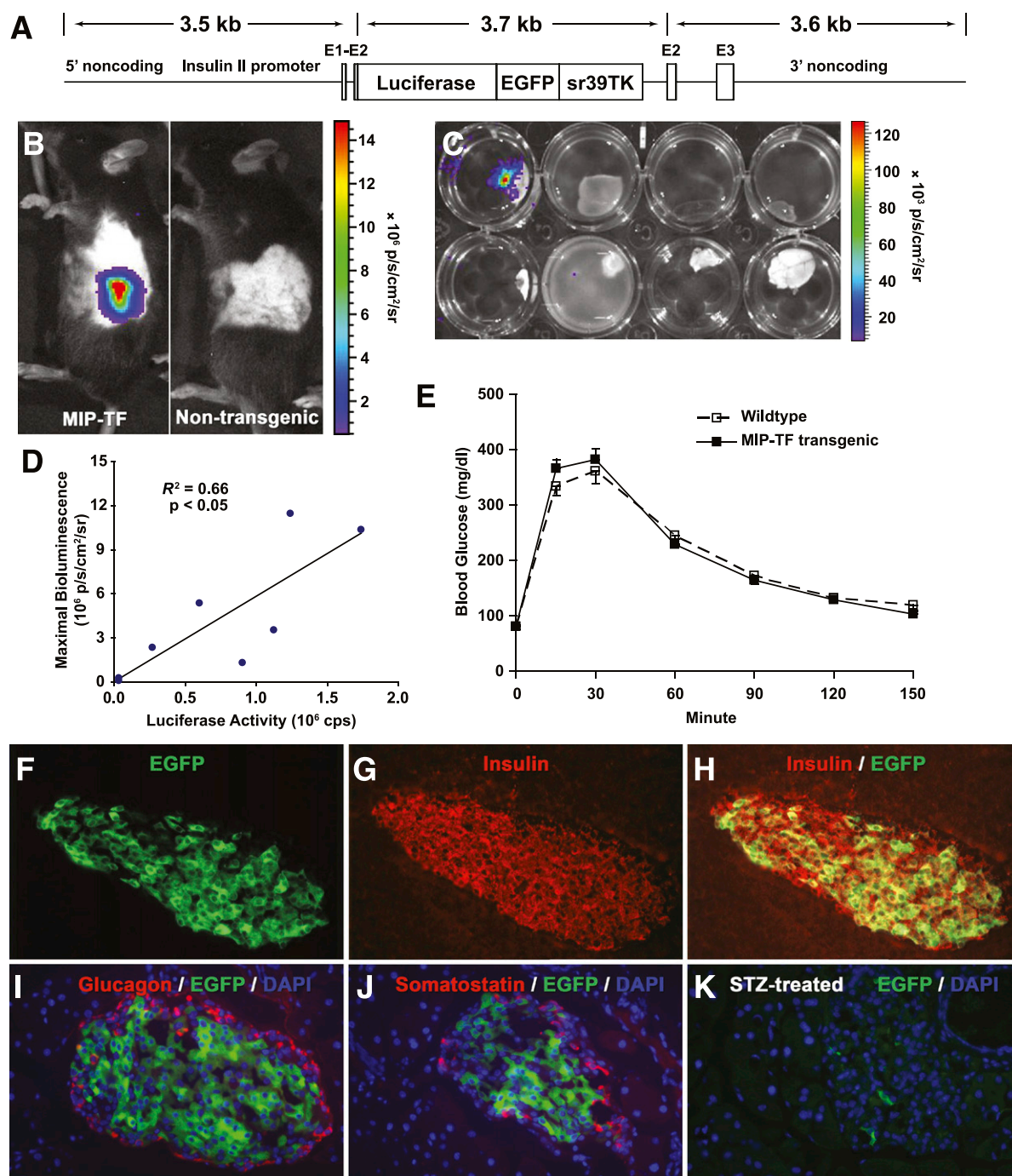
FIG. 1. Generation and characterization of MIP-TF mice. A: Diagrammatic representation of the construct used for microinjection. The trifusion reporter cDNA (firefly luciferase/EGFP/truncated HSV1-sr39TK) (15) is flanked on its 5' end by 3.5 kb of genomic DNA upstream of the mouse insulin II ATG translational start site and, on its 3' end, has 3.6 kb of genomic DNA that lies immediately 3' of the ATG translational start site of insulin II. Exons of the insulin II gene are indicated as E1–3. B: Bioluminescence was detected specifically from the pancreas region of line 300 mice (referred to as MIP-TF mice; at left), but not a nontransgenic littermate (at right). The sides of both mice were shaved to maximize detection of bioluminescence. C: Representative BLI of freshly dissected organs from a MIP-TF mouse after luciferase injection. Top row (left to right): pancreas, liver, spleen, and heart; bottom row (left to right): lung, thymus, muscle, and brain. D: In vivo bioluminescence (measured as maximal radiance) showed a linear correlation with luciferase activity in pancreas homogenates ( R^2 = 0.66 , P < 0.05 ). E: IPGTT test. Data shown are the mean blood glucose levels after glucose challenge \pm SEM; n = 14 mice/group. F–H: Expression of EGFP in \beta -cells of MIP-TF mice. Pancreas sections from MIP-TF mice were immunostained for insulin (red) and examined for EGFP expression (green) by fluorescence microscopy. Only insulin-positive cells also expressed EGFP. There was no overlap of EGFP expression (green) with glucagon (red; I ), or somatostatin ( J ). Islets from mice rendered diabetic with STZ had few or no EGFP-expressing islet cells ( K ). (A high-quality color representation of this figure is available in the online issue.)
