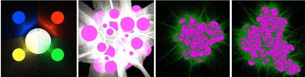
Fig. 1: Example results: (a) A single Voronoi cell pictured, where the green Voronoi vertex is equidistant from the 5 spheres; the full Voronoi diagram we computed for (b) "Random Set A" [12]; (c) Protein ID 1crn-PQR consisting of 642 atoms (202 Cs, 55 Ns, 64 Os, 6 Ss, and 315 Hs) [14]; (d) Protein ID 1bh8-PQR consisting of 2161 atoms (680 Cs, 181 Ns, 203 Os, 10 Ss, and 1087 Hs) [14].
