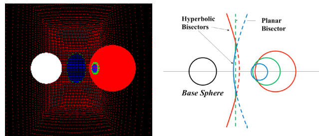
Fig. 7: Special case of Jacobian singularity when bisectors do not actually intersect (Input consists of 3 intersecting colored spheres and a white base sphere; a cross section is also shown).
