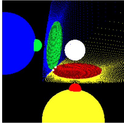
Fig. 8: Case of a non-converging grid cell with two intersections. The two Voronoi vertices (white) are at the intersection of the same four bisectors (blue, green, red, and yellow).
