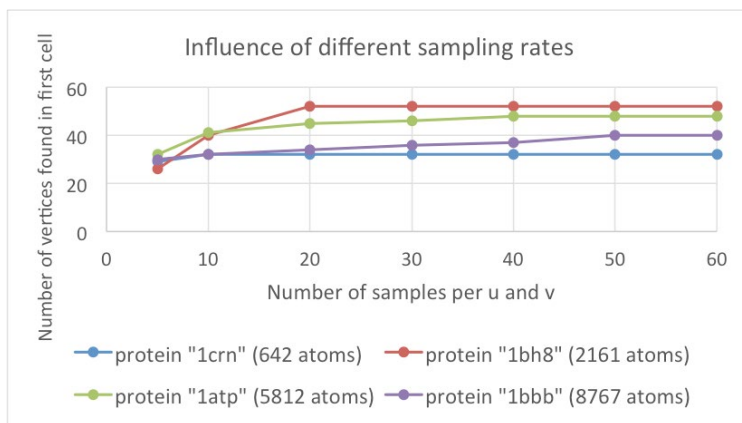
Figure 13: Sampling rate vs. the number of vertices calculated.
