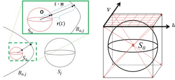
Fig. 2: (a) Illustration of ray intersection with bisector surfaces. (b) Mapping sphere to six u-v parametric surfaces on the bounding cube; uniform parametric sampling of top surface shown.
