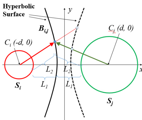
Fig. 3: Culling the incorrect sheet of the two hyperboloid sheets.
