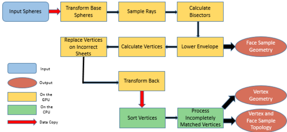
Fig. 12: GPU framework.
