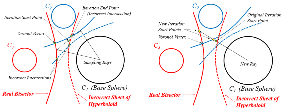
Fig. 10: (a) Converging to an incorrect intersection with an unnecessary sheet of the bisectors. (b) Finding new start points for Newton-Raphson method.
