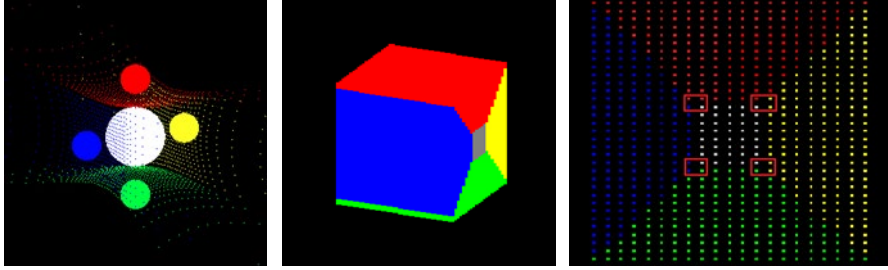
Fig. 5: (a) Sample points on Voronoi faces for white base sphere; (b) Corresponding color map of u-v domains on bounding cube; (c) Sample point grid on one face of the bounding cube with 3-color grid cells indicated.
