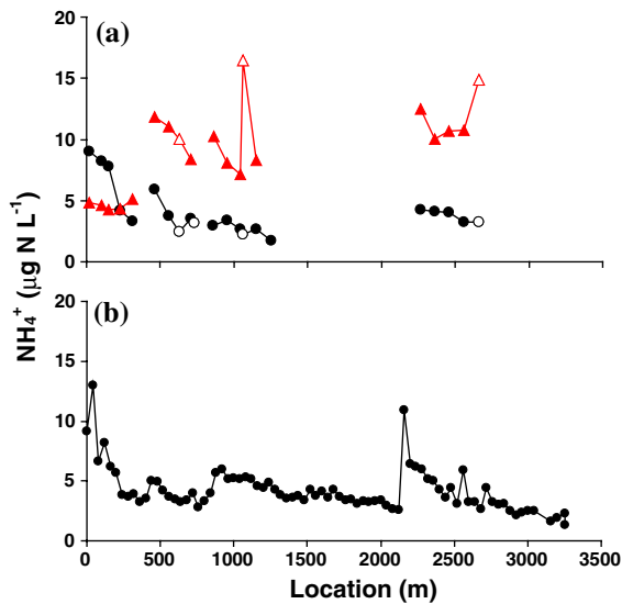
Fig. 3 a Background \text{NH}_4^+ concentrations for reach sampling locations; b Background \text{NH}_4^+ concentrations for detailed synoptic (40 m) for fall 2003. Circles are fall 2003; triangles are summer 2004; open symbols are debris dam reaches
