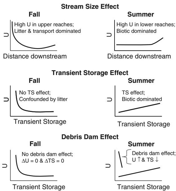
Fig. 6 Summary of the effect of stream size, transient storage and debris dams on \text{NH}_4^+ uptake rate
