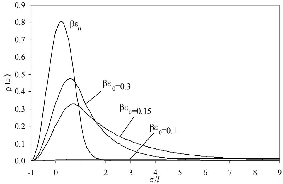
Fig. 4 Effect of energy \varepsilon_0 on the density distribution of a polymer in the square well.
