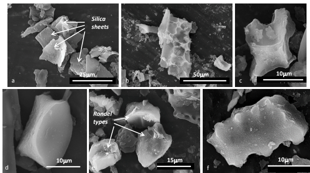
Figure 1. SEM images of TD-F-L wheat phytolith assemblage, deposited on an aluminum mount. Three categories are illustrated: (1) silica sheets ( a , b ), (2) stellate type from intercellular space ( c ) and (3) GSC phytoliths including rondel ( d , e ) and polylobate types ( f ).
