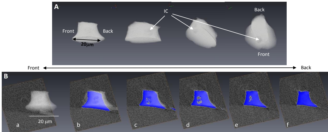
Figure 4. 3-D X-ray microscopy of a GSC phytolith from wheat (TD-F-L): (a) four views of the reconstructed volumes; internal cavities (IC) are distinguishable. (b) 2-D X-ray slices superimposed on the phytolith volume rendering, showing from front to back the internal cavity (IC). No connection to the surface was evidenced. The blue area corresponds to the thresholding of the phytolith grayscale values.
