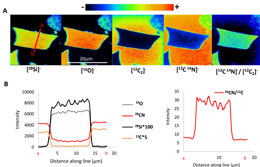
Figure 6. NanoSIMS images and intensities of a first typical GSC phytolith (rondel type) from TD-F-L (wheat) embedded in epoxy resin (polished section). Pre-sputtering: L1 = 2 kV de-focused ( 60 \times 60 mm) [\text{Cs}]^+ primary beam, for 3 min (a) [\text{Si}^{28}]^- , [\text{O}^{16}]^- , [\text{C}_2^{12}]^- , [\text{C}^{12}\text{N}^{14}]^- and [\text{C}^{12}\text{N}^{14}]^- / [\text{C}_2^{12}]^- images obtained with a [\text{Cs}]^+ primary beam with L1 = 2 kV, D1-1 primary diaphragm ( 750 \mu\text{m} ), for 11 min; (b) secondary ion intensities along line scans (red line in a).
