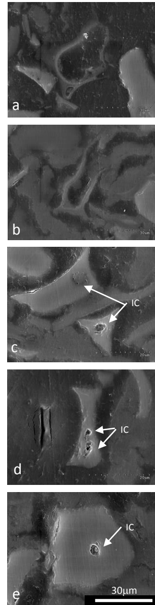
Figure 2. SEM images of the thin section of the TD-F-L wheat phytolith types including silica sheets ( a , b ), and GSC phytoliths of the rondel type ( c , d , e ). GSC types show micrometric internal cavities (IC).
