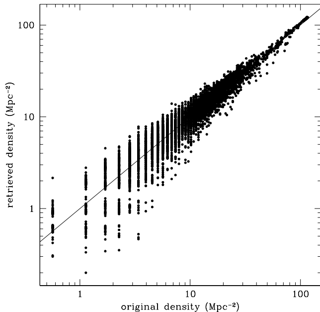
Figure 2. Comparison between the original local density estimated in the Kitzbichler & White (2007) mock catalogues and the density retrieved in the randomly extracted catalogue following our method. The solid line shows the 1-to-1 relation.
