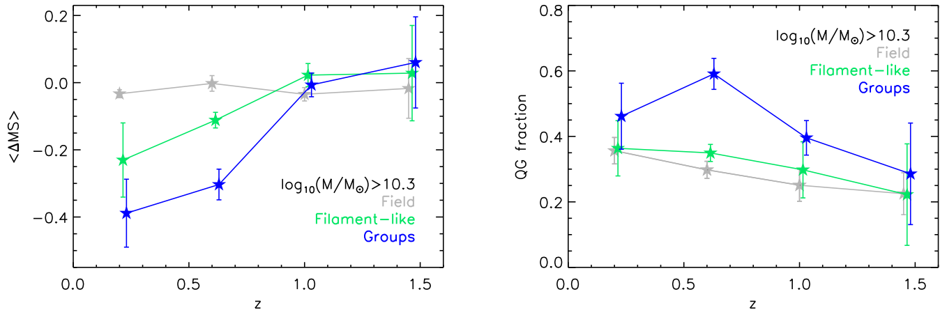
Figure 11. Left: Evolution of the MS offset for group, “filament-like” and field star-forming galaxies with M_{\star} > 10.3 . \Delta MS represents the central value of the residuals with respect to the predicted MS for each redshift bin. Right: Evolution of the quiescent galaxy fraction ( f_{QG} ) for group (blue stars), “filament-like” (green stars) and field (grey stars) galaxies with M_{\star} > 10.3 . We define “quiescent” all the galaxies with \Delta MS < -1 . In both panels errors are derived using the mock catalogues of Kitzbichler & White (2007), as explained in the text and data points are artificially shifted for clarity.
