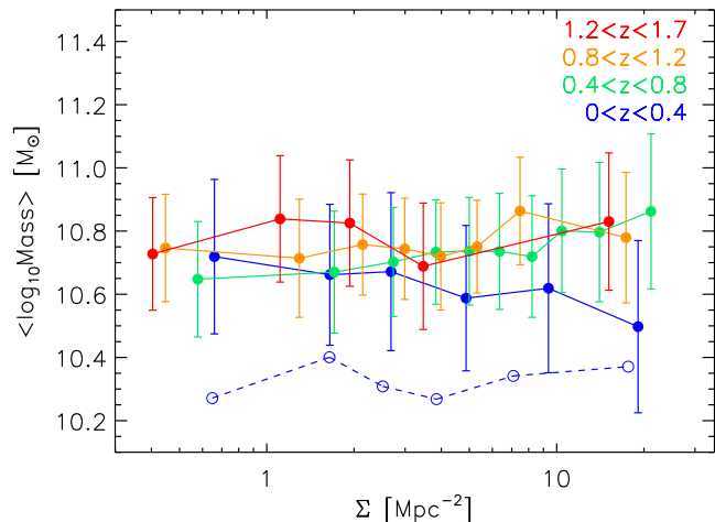
Figure 5. Stellar mass–density relation for all the galaxies with M_{\star} > 10^{10.3} M_{\odot} in different redshift bins (solid lines). Errors are derived using the mock catalogues of Kitzbichler & White (2007), as explained in the text. The dashed line represents the M_{\star} –density relation at 0 < z < 0.4 for all galaxies with M_{\star} > 10^9 M_{\odot} . The normalisation of the dashed line is artificially increased to higher value to make it close to the blue solid line and make the comparison easier.
