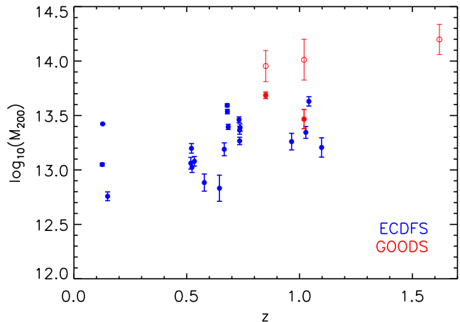
Figure 1. M_{200} as a function of redshift for all groups considered in our sample. Filled circles represent the X-ray mass estimates, while empty circles show the dynamical mass estimates. We highlight in blue the ECDFS sample and in red the GOODS groups.
