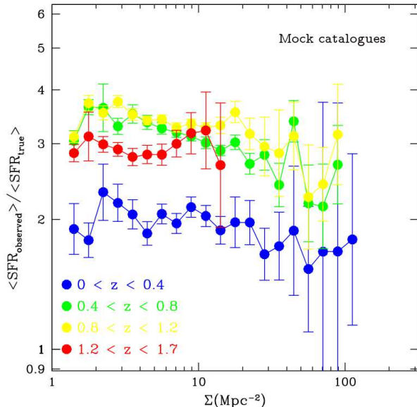
Figure 6. Ratio between the SFR derived from the incomplete mock catalogues ( \langle \text{SFR}_{\text{observed}} \rangle ) and the SFR from the complete ones ( \langle \text{SFR}_{\text{true}} \rangle ) versus density for all four redshift bins used in this work. We do not find any bias in the slope of the SFR–density relation of Fig. 4 as confirmed by the Spearman test.
