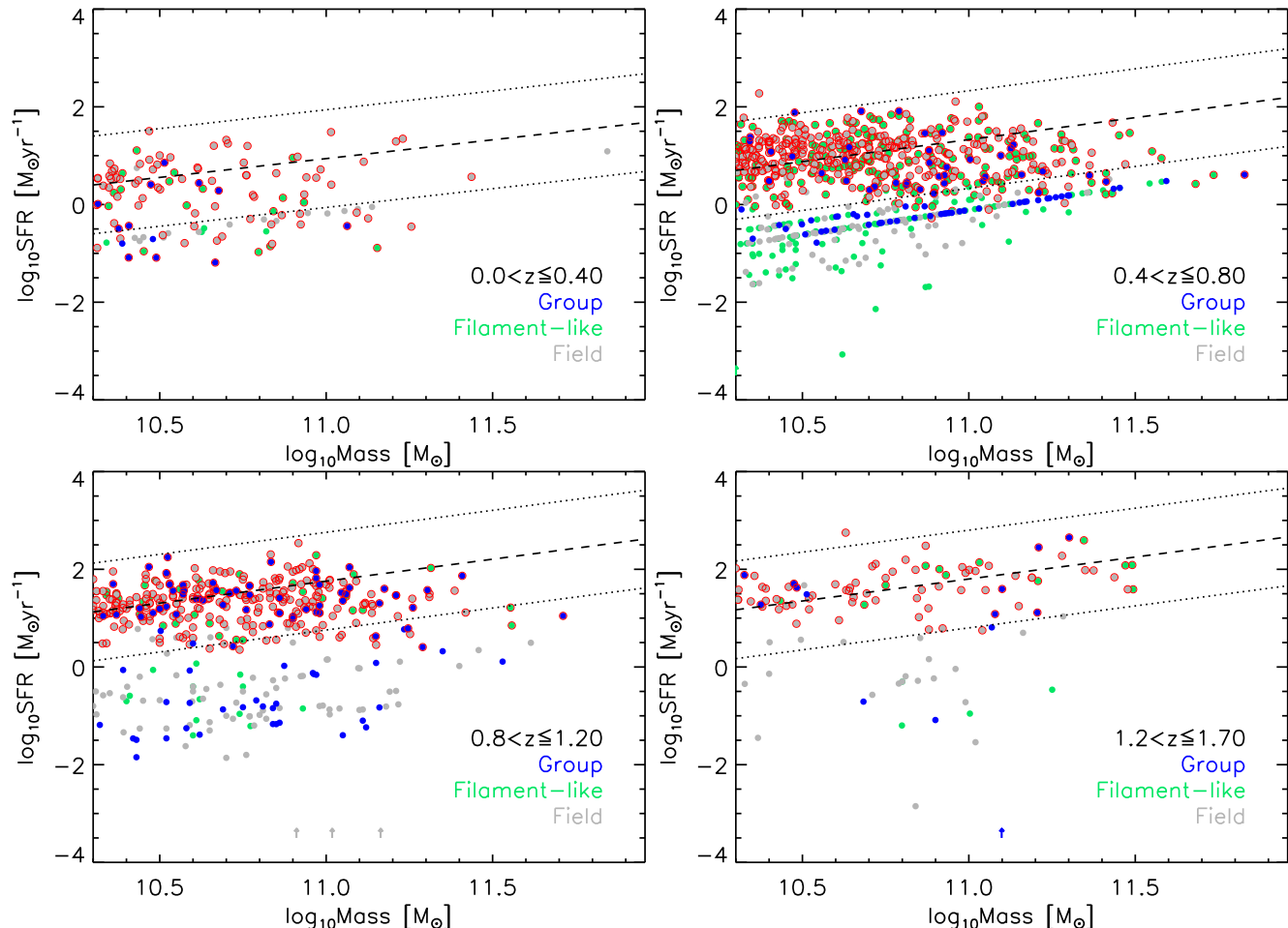
Figure 10. SFR – M_* diagrams for the different redshift bins considered in this work. We distinguish between group (blue filled circles) “filament-like” (green filled circles) and field (grey filled circles) galaxies. The empty red circles represent all galaxies detected in the IR bands. The dashed lines show the MS relations from the literature as explained in the text. MS galaxies are selected within the dotted lines, while QG are found below the dotted line, at lower SFR. The upward pointing arrows represent lower limits.
