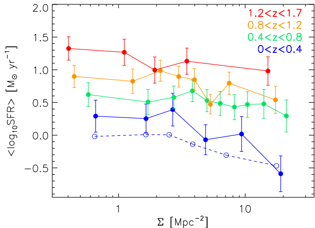
Figure 4. SFR–density relation for galaxies with M_{\star} > 10^{10.3} M_{\odot} in different redshift bins (solid lines). The dashed line represents the SFR–density relation at 0 < z < 0.4 for all galaxies with M_{\star} > 10^9 M_{\odot} . Errors are derived using the mock catalogues of Kitzbichler & White (2007), as explained in the text.
