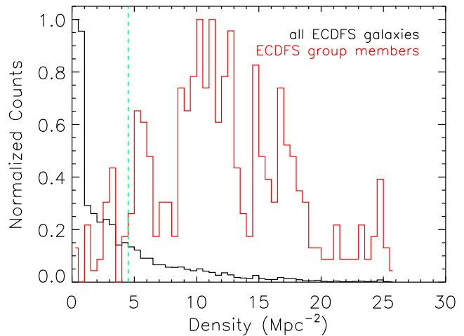
Figure 3. In black: density distribution around each galaxy with a spectroscopic redshift in ECDFS. The red histogram shows the density of group members. The green dashed line at 4.5 galaxies \text{Mpc}^{-2} nicely separates the group-dominant regime from the field-dominant regime. Indeed, 75% of field galaxies are found at densities below this threshold and 92% of group galaxies above that.
