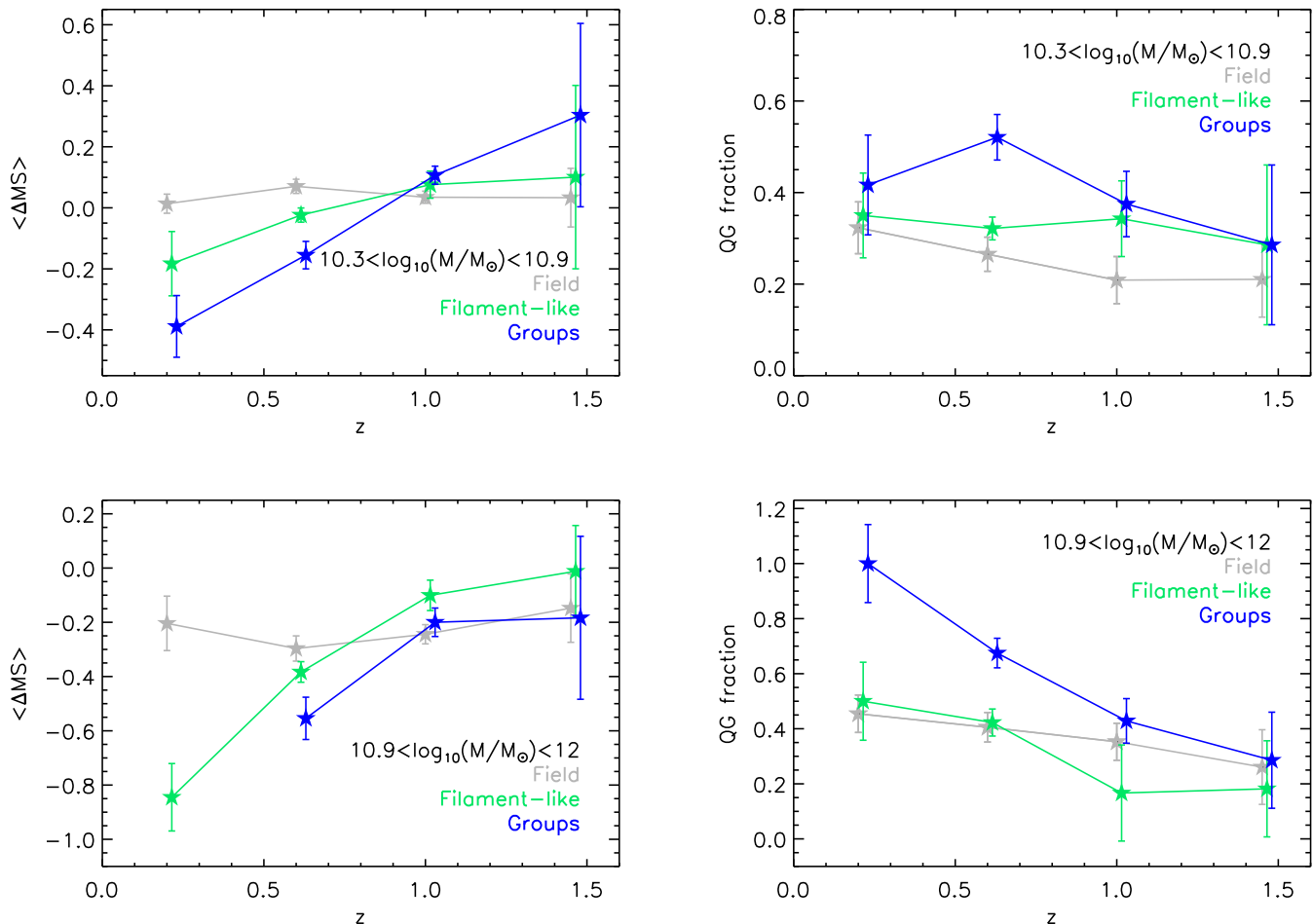
Figure 12. Left column: Evolution of the MS offset for group, “filament-like” and field star-forming galaxies with 10.3 < \log(M_{\star}/M_{\odot}) < 10.9 and 10.9 < \log(M_{\star}/M_{\odot}) < 12 (top and bottom, respectively). Right column: Evolution of f_{QG} for group (blue stars), “filament-like” (green stars) and field (grey stars) galaxies for the same range of stellar mass as in the left column. In all panels errors are derived using the mock catalogues of Kitzbichler & White (2007), as explained in the text and data points are artificially shifted for clarity.
