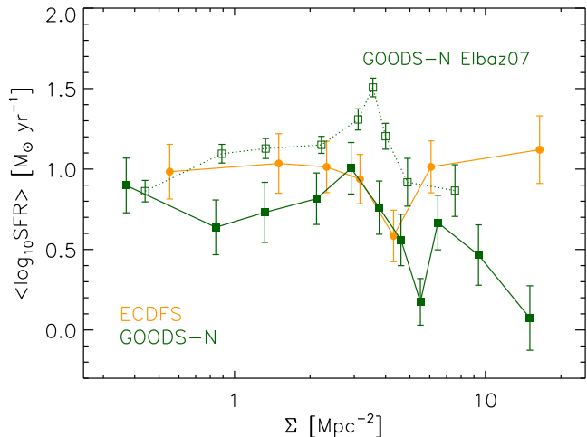
Figure 7. SFR–density relation for all galaxies with M_{\star} > 10^{10.3} M_{\odot} at z \sim 1 . Galaxies in the ECDFS and GOODS-N fields are shown in orange and green, respectively. The open symbols connected by a dotted line show the SFR–density relation of Elbaz et al. (2007) for GOODS-North.
