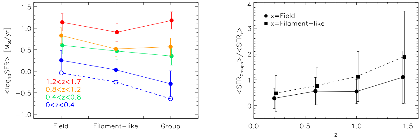
Figure 8. Left: Comparison of mean SFR among group (within 2 \times R_{200} ), “filament-like” and field galaxies. Errors are derived using the mock catalogues of Kitzbichler & White (2007), as explained in the text. The dashed line represents the mean SFR for the different environments at 0 < z < 0.4 for all galaxies with M_{\star} > 10^9 M_{\odot} . Right: ratio between the \langle \text{SFR} \rangle of group galaxies with respect to field and “filament-like” galaxies as a function of redshift. In both panels data points are artificially shifted for clarity.
