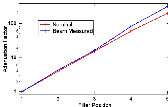
Figure 4: Calibration of the filter-attenuation system.
