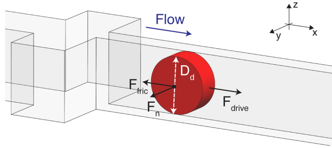
Supplementary Figure 5, related to Figure 2. Schematic drawing of the forces around the deformed cell while in the contraction channel. F_{\text{drive}} , F_n , F_{\text{fric}} , and D_d correspond to the driving force, normal force, frictional force, and the diameter of the deformed cell while in the contraction channel, respectively. Under a cell's constant velocity, the driving force generated by the pressure difference around the cell is counter-balanced by the frictional forces between cell surface and the channel wall.
