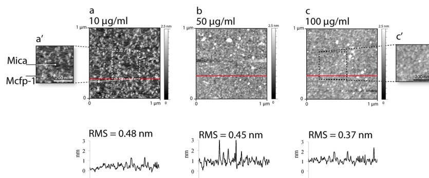
Figure 4. Mfp-1 ( Mc ) films adsorbed to mica. AFM topography images and their respective cross sections (below) showing the RMS roughness of mfp-1 ( Mc ) films on mica in pH 5.5 acetate buffer at different C_{fp1} = (a) 10, (b) 50, and (c) 100 \mu\text{g}/\text{mL} .
