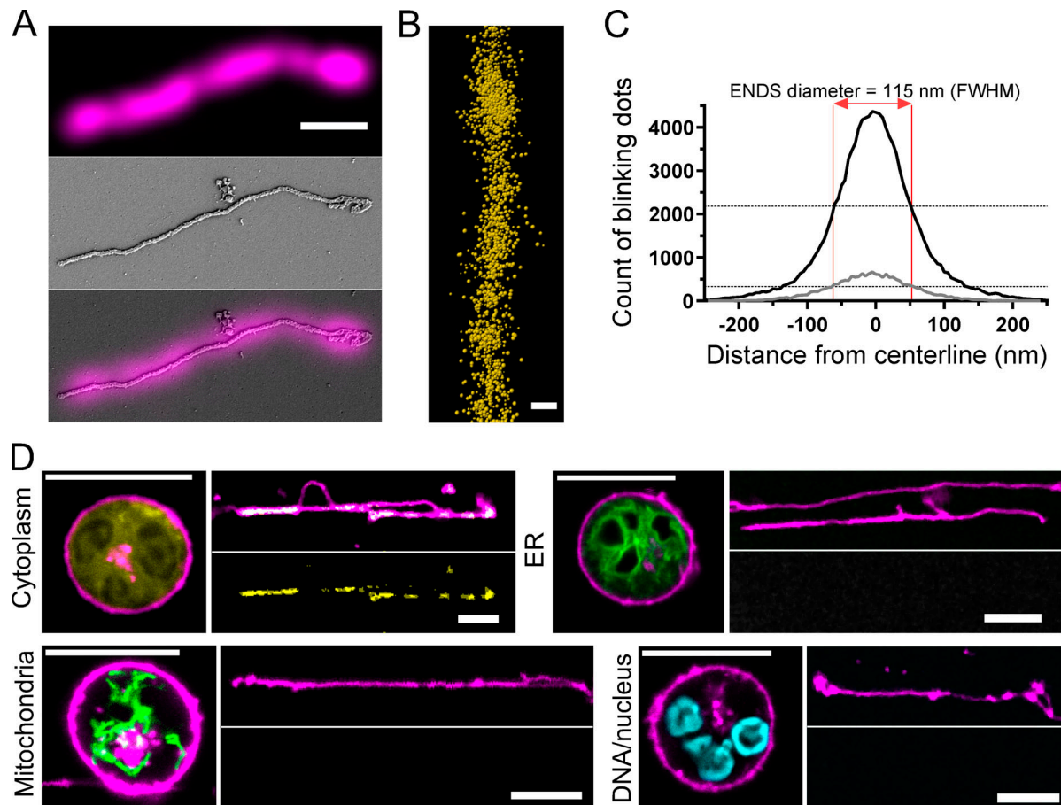
Figure 2. Structure and composition of human ENDS. (A) SEM and confocal image of ENDS formed on P-selectin substrate by human neutrophils surface labeled with CD16-AF647 antibody (magenta). Scale bar, 1 \mu\text{m} . (B) ENDS formed on E-selectin labeled with CD16-AF647 antibody were analyzed with STORM. Image shows a section of ENDS. Dots indicate the localization of the labeling antibody detected with STORM. Certainty of localization \leq 20 nm. Scale bar, 100 nm. (C) The frequency histogram shows the distribution of CD16-AF647 labeling antibody across the width of ENDS measured as in B. Data were collected from two independent experiments (black and gray curves). The distance between the vertical red lines indicates mean ENDS diameter determined as the full width at half maximum (FWHM) value. Bin size is 5 nm. (D) To test the presence of organelles in ENDS, neutrophils were labeled for their surface (CD16-AF647 antibody, magenta), cytoplasm (CellTracker Orange CMRA, yellow), ER (ER Tracker Green), mitochondria (Mito Tracker Green), or nucleus/DNA (Hoechst, cyan) and rolled on E-selectin substrate. Only the cytoplasm tracer was detectable in ENDS formed by these neutrophils. Scale bars, 10 \mu\text{m} . Each of the experiments shown on this figure were repeated at least twice.
