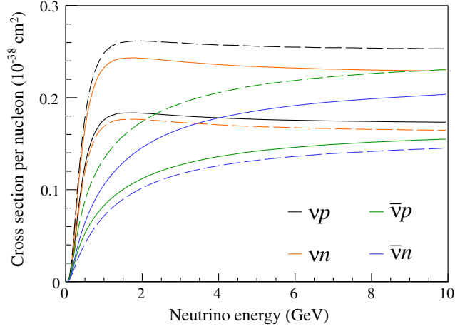
FIG. 1. NCQE cross section on carbon per nucleon as a function of neutrino energy. The black and orange lines represent the neutrino cross sections on protons and neutrons, respectively. The green and blue lines represent the antineutrino cross sections on protons and neutrons, respectively. The solid (dashed) lines are the cross sections with g_A^s = 0 ( -0.3 ). These results are obtained using NuWro with M_A = 1.2 GeV [10].
