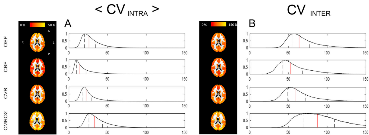
Fig. 5. Voxel-wise CV indices calculated from the within-session dataset. A: results for \langle CV_{\text{intra}} \rangle , the mean across subjects of the intra-subject CV. B: results for CV_{\text{inter}} , the inter-subject CV. For both, reported are the axial views of the calculated maps for each physiological parameter and relative histograms showing the distributions of the calculated values (in red the median and in black the interquartile range limits).
