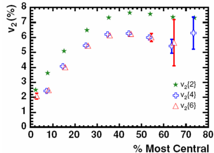
Fig. 7 Many particle cumulant results for charged hadron v_2 from \sqrt{s_{NN}} = 130 GeV Au+Au as a function of centrality [21].
