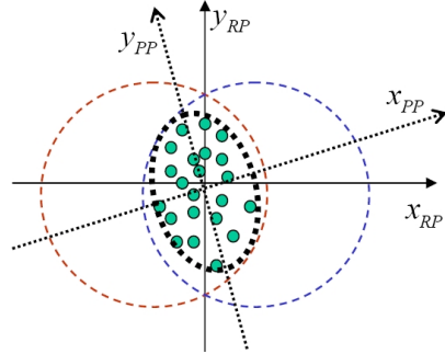
Fig. 2 The definitions of the Reaction Plane and Participant Plane coordinate systems.
