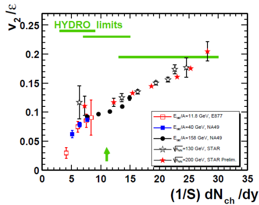
Fig. 19 Compilation of v_2/\epsilon data [4] vs particle density at midrapidity. Green lines indicate ideal hydrodynamic predictions for AGS, SPS and RHIC collision energies [71].
