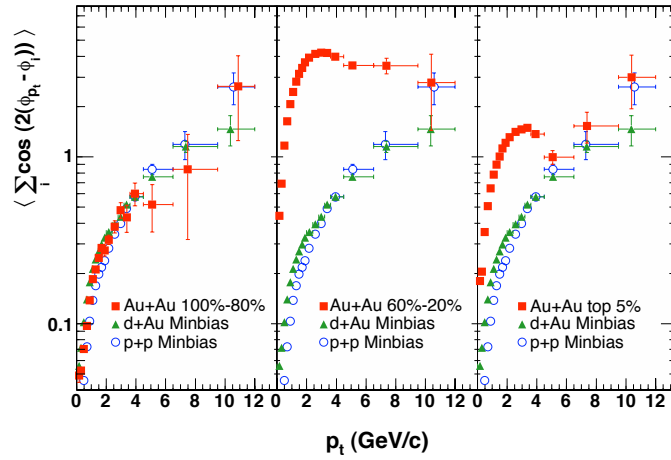
Fig. 44 Azimuthal correlations in p+p, d+Au, and Au+Au collisions of different centralities [26, 129].
