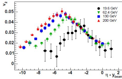
Fig. 32 v_2 as a function of \eta - y_{beam} at four collision energies [100]. The data were obtained with the eta subevent method.
