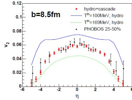
Fig. 33 Pseudorapidity dependence of elliptic flow from PHOBOS compared to a hydro+cascade model [75]. The lines are for sudden freeze-out at different temperatures. The data were obtained with the eta subevent method.
