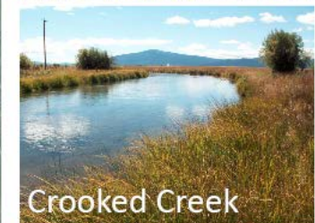
Figure 3. Approximate gage station locations for the Wood River, Fort Creek, and Crooked Creek in the UKL Sub-Basin, Oregon.
