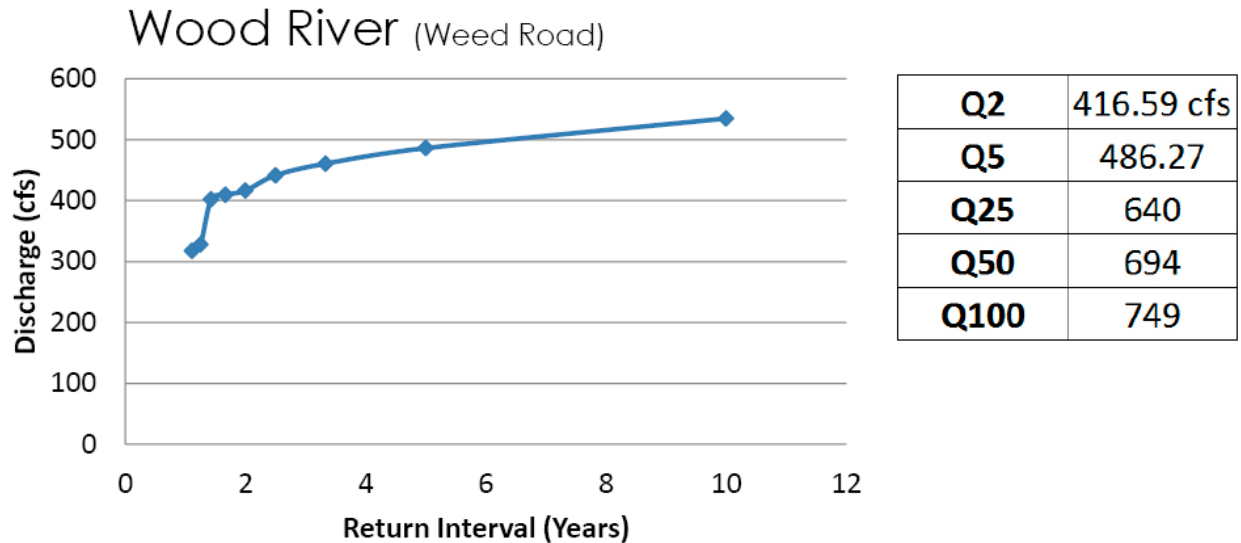
Figure 11. Measured annual peak flows and estimated re-occurrence intervals for the Wood River at Weed Road from 10/6/2004-3/26/2012.
