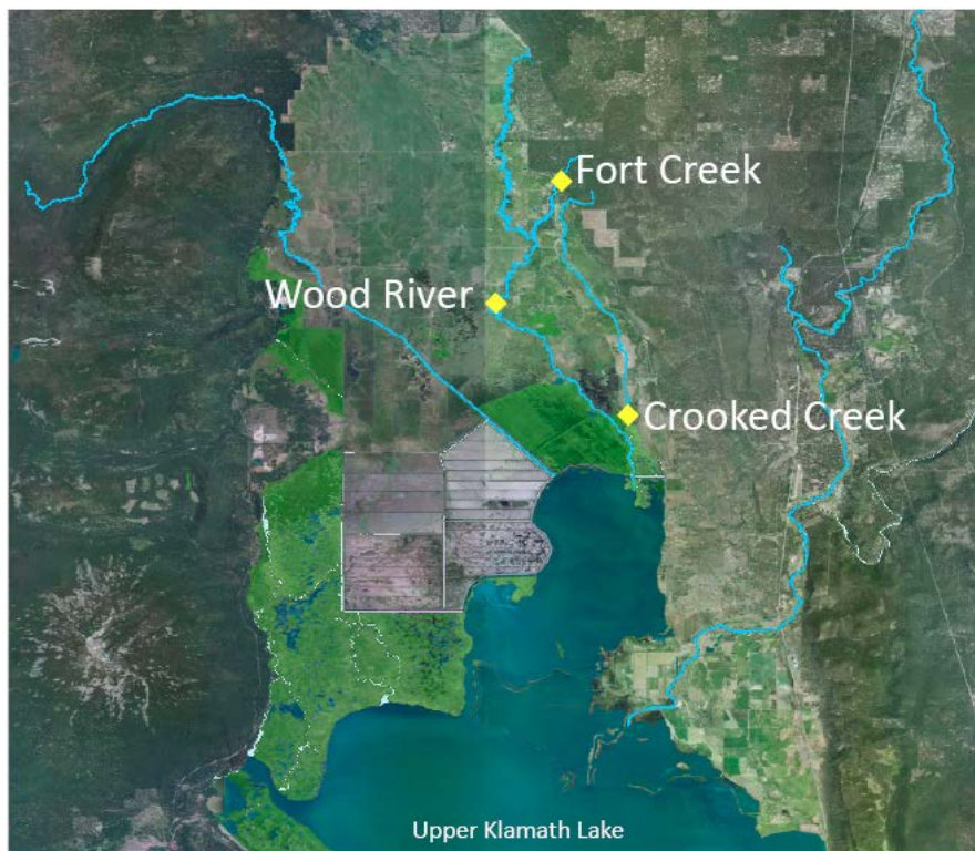
Figure 3. Approximate gage station locations for the Wood River, Fort Creek, and Crooked Creek in the UKL Sub-Basin, Oregon.
