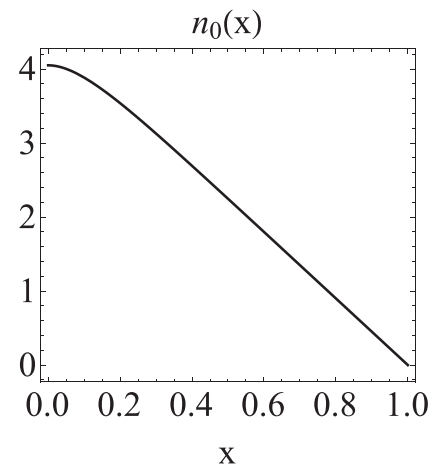
FIG. 13. Initial density profile given by the function n_0(x) in Eq. (55) ( b = 20 ), for g_i = 4.5 .
