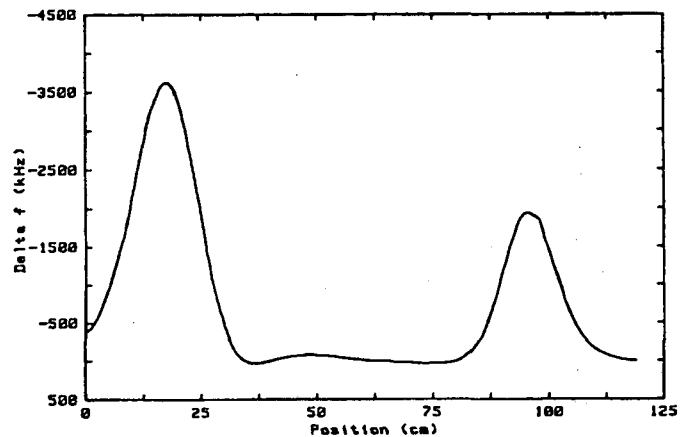
Figure 2e: TM_{011-0} Exp Mode.
