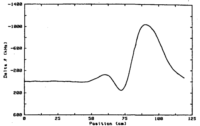
Figure 2d: TE_{111} Exp B.L.H.
