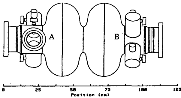
Figure 1: Cavity Geometry.
