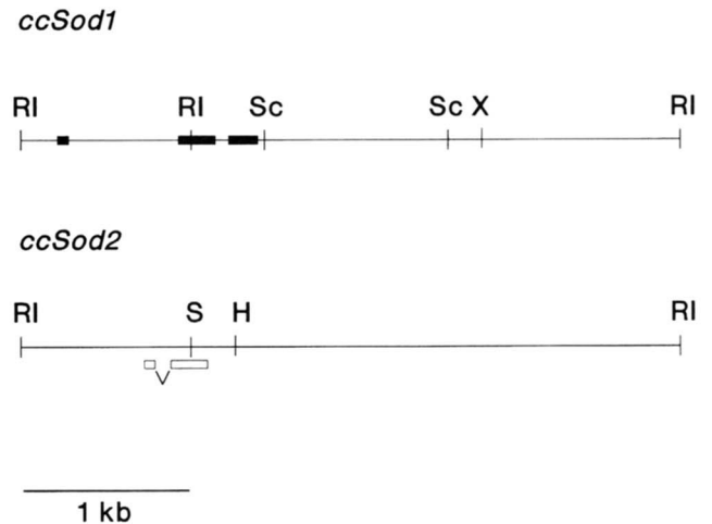
FIGURE 2.—Restriction maps of the ccSod1 and ccSod2 genes in Ceratitis capitata . The restriction map of ccSod1 , with the exons shown as solid boxes, is taken from KWIATOWSKI et al. (1992). The probe for ccSod1 was a 4-kb clone, whereas the probe for ccSod2 was a 330-bp cDNA fragment generated by primers I and IIIb (shown on the figure as two open boxes). Restriction enzymes are RI, EcoRI ; Sc, ScaI ; X, XbaI ; S, Sall ; H, Hind III .
