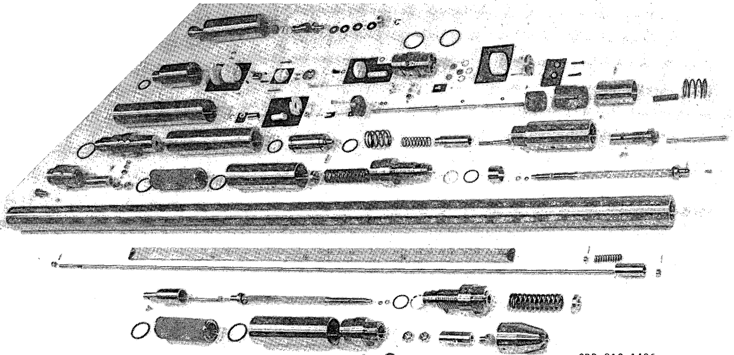
Figure 2. The disassembled sampler.
