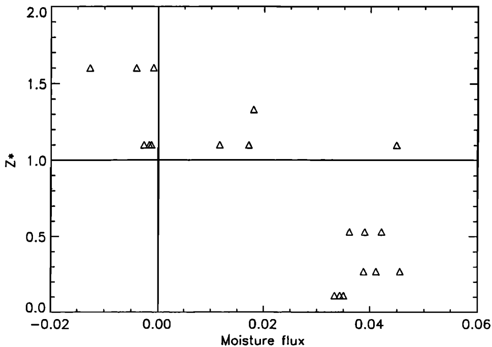
Figure 11. Humidity flux from wavelengths <5.3\mu , measured within and above the boundary layer. The highest fluxes above the boundary layer are associated with large patches of clouds.
