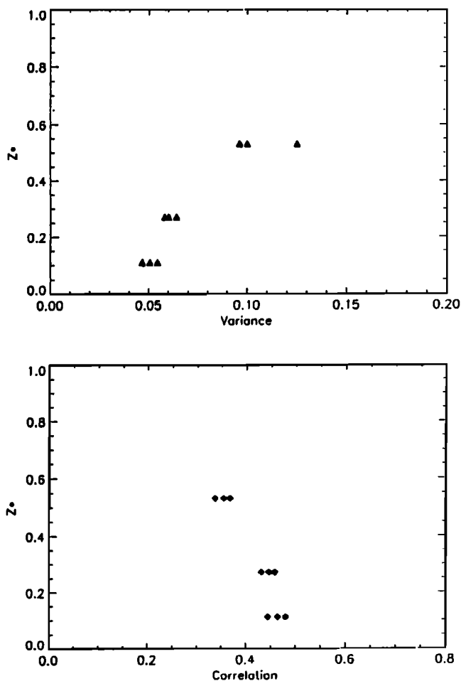
Figure 7. The humidity variance (\sigma_q)^2 ( \text{g kg}^{-1} ) 2 and the correlation coefficient F_q/(\sigma_w\sigma_q) for wavelengths < 5.3z_i . Each data point represents the variance calculated from high-rate data during one constant-altitude circle. The data were collected from 0530 to 1330 local time (1536–2330 UTC). The highest variance value (0.125 at z_* = 0.53 ) comes from the first circle 0536–0602 local time.
