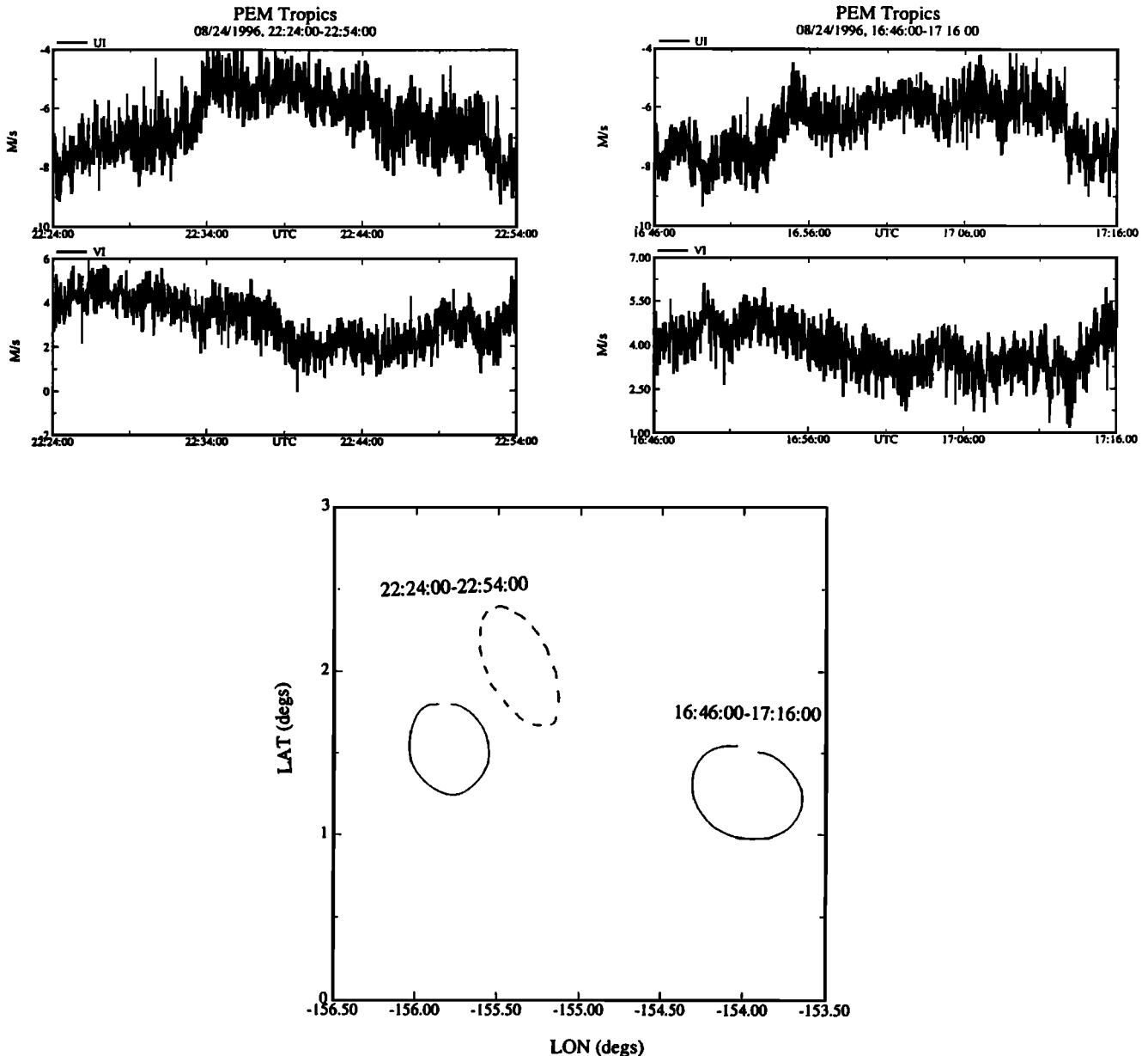
Figure 14. Variations in the east and north wind components (UI and VI) during two clockwise circles, 5 hours 40 min apart, at z_* = 0.27 . Below is the flight track (solid lines). The dashed line shows the approximate position of the earlier circle 5 hours 40 min later assuming it is advected with the wind observed during the earlier circle. One degree \approx 100 km.
