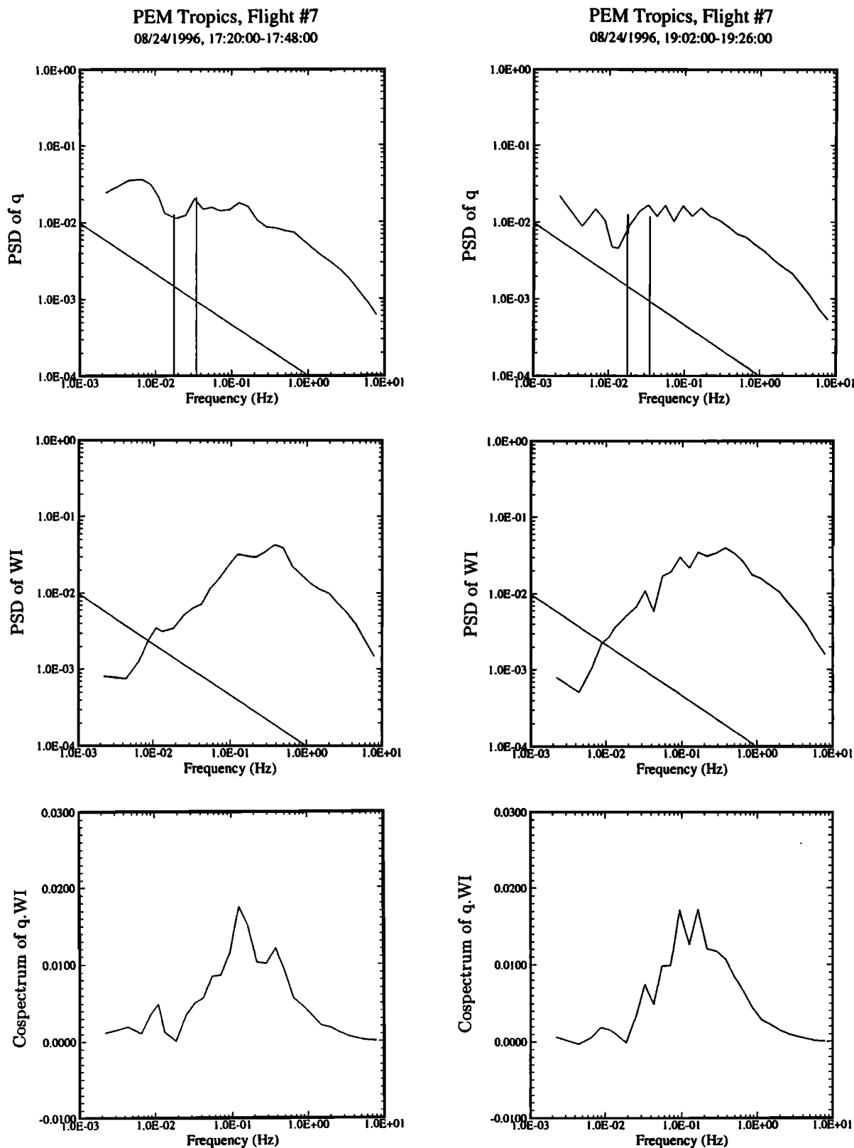
Figure 6. Mesoscale contributions to power spectra (PSD) times frequency of specific humidity ( q , g^2 kg^{-2} ), vertical velocity ( WI , m^2 s^{-2} ), and their cospectra. The plots are based on high-rate data, collected at about 18 samples/s, during the first two circles at z_* = 0.11 . The diagonal line in the power spectra plots shows the 2/3 slope, characteristic of turbulence in the inertial subrange. The two vertical lines on the q power spectra mark frequencies at 10z_i and 5z_i .
