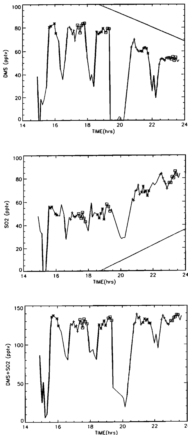
Figure 3. Changes in DMS and \text{SO}_2 concentrations with time (UTC). The local solar time is 10 hours earlier. The squares, crosses, and asterisks represent 5 min data samples from circles in the boundary layer where the normalized altitude z_* is 0.11, 0.27, and 0.53, respectively. Lower DMS and \text{SO}_2 concentrations were observed above the boundary layer. To avoid clutter, these samples are not marked by symbols. The straight line shows the diurnal changes in DMS and \text{SO}_2 , estimated so as to minimize variance in the normalized data set.
