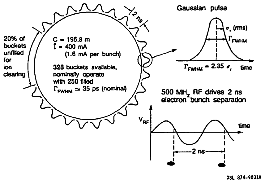
Fig. 3. Schematic illustration of the electron bunch structure in the ALS storage ring during multibunch operation. As shown at the upper right, each bunch has a full width at half maximum of about 35 ps. The spacing between bunches, dictated by the rf frequency, is 2 ns.
