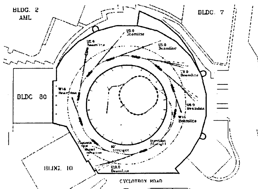
Fig. 13. Floor plan showing a possible placement of insertion devices and locations of associated beamlines in the ALS building. The maximum beamline length is about 35 m. The prime bend-magnet ports to be developed initially are located in the center bend magnet of each storage-ring arc. At two ports per magnet, there is a total of 24 ports.
