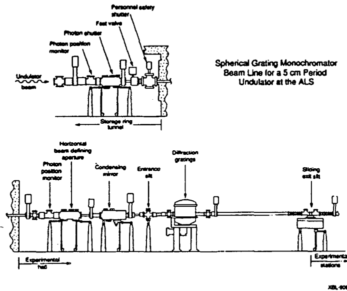
Fig. 11. Beamline layout for the US.0 beamline. The front end inside the storage-ring shield wall is shown on the top; the branchline outside the storage-ring shield wall is shown on the bottom. User-supplied optics beyond the monochromator and the experimental stations are not shown.
