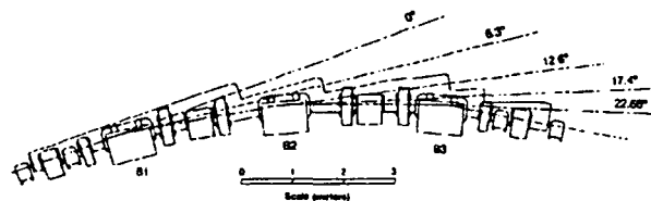
Fig. 2. Arrangement of photon-beam ports in one superperiod of the ALS storage-ring lattice showing an insertion-device port and four bend-magnet ports.
