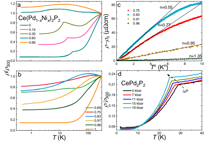
FIG. 5. (a) and (b) The electrical resistivity normalized to the room temperature value \rho/\rho_{300K} vs. temperature T for Ce(Pd 1-x Ni x ) 2 P 2 at values x = 0 - 1 . (c) Power law fits to the low temperature electrical resistivity for selected concentration of Ce(Pd 1-x Ni x ) 2 P 2 near x_{cr} . (d) \rho/\rho_{300K}(T) collected under applied pressure P \lesssim 19 kbar for CePd 2 P 2 .
