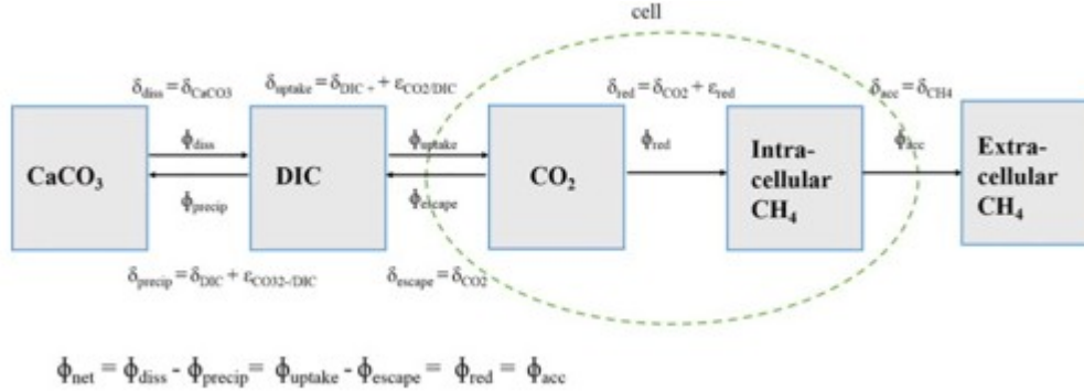
Fig. 4. Steady state model illustrating the various carbon fluxes and their isotopic compositions in the \text{CaCO}_3 experiments. From left to right: calcium carbonate dissolves ( \phi_{\text{diss}} ) and carbon accumulates in the dissolved inorganic carbon (DIC) pool from where the carbonate ( \text{CO}_3^{2-} ) species can re-precipitate ( \phi_{\text{precip}} ) and the \text{CO}_2 species can diffuse into the cell ( \phi_{\text{uptake}} ) and back out ( \phi_{\text{escape}} ) unless it is converted into \text{CH}_4 ( \phi_{\text{red}} ) and subsequently accumulates in the extracellular medium and headspace. The measured isotopic composition is that of the accumulated extracellular \text{CH}_4 , which was sampled from the headspace. The small isotopic effects associated with \text{CH}_4 diffusion through water and partitioning between dissolved and gaseous \text{CH}_4 do not have a significant effect and are excluded for clarity.
