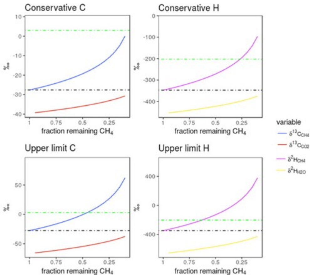
Fig. 6. Expected changes in \delta^{13}\text{C} and \delta\text{D} of residual \text{CH}_4 during incremental closed-system oxidation under two different fractionation factors scenarios. Initial value of \delta^{13}\text{C} is -27.6\text{‰} and \delta\text{D} is -347\text{‰} , as indicated by the solid black lines. Conservative C fractionation factor \alpha_{\text{CH}_4/\text{CO}_2} is 1.012 ( =12\text{‰} ) and upper limit \alpha_{\text{CH}_4/\text{CO}_2} is 1.039 ( =39\text{‰} ). Conservative H fractionation factor \alpha_{\text{CH}_4/\text{H}_2\text{O}} is 1.109 ( 109\text{‰} ) and upper limit H \alpha_{\text{CH}_4/\text{H}_2\text{O}} is 1.315 ( 315\text{‰} ). Fractionation factors are taken from Holler et al. (4). Dashed green lines indicate the \delta^{13}\text{C} and \delta\text{D} values of methane ( +3\text{‰} and -200\text{‰} , respectively) that have been measured from subsurface fluids rich in \text{CH}_4 in an Oman hyperalkaline serpentinite aquifer. The isotopic composition shown for the accumulated product ( \text{CO}_2 and \text{H}_2\text{O} , respectively in blue) represents only the pool released from methane oxidation and not any mixing with pre-existing sources of \text{CO}_2 and \text{H}_2\text{O} .
