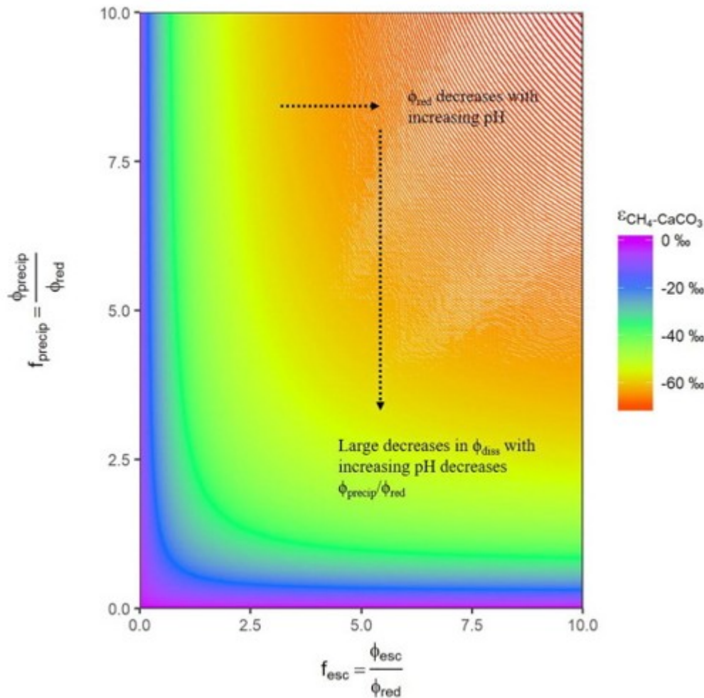
Fig. 5. Range of \epsilon_{\text{CH}_4\text{-CaCO}_3} values obtained from varying the rate of \text{CO}_2 escape from the cell ( \phi_{\text{escape}} ) and the rate of carbonate re-precipitation ( \phi_{\text{precip}} ) both relative to the methane production rate ( \phi_{\text{red}} ).
