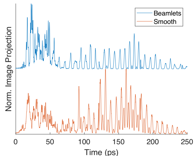
Fig. 9 | Normalized EOS measurements of temporal intensity for smooth and beamlet distributions at \gamma = 16.3 .
