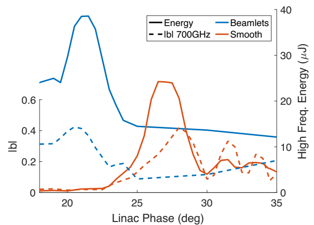
Fig. 8 | GPT simulations of longitudinal compression. The energy and magnitude of the bunching factor for smooth and beamlet distributions are plotted versus the RF linac phase where 0° corresponds to the maximum energy setpoint. The bunching is computed for the 700 GHz phase resonance at the undulator entrance.
