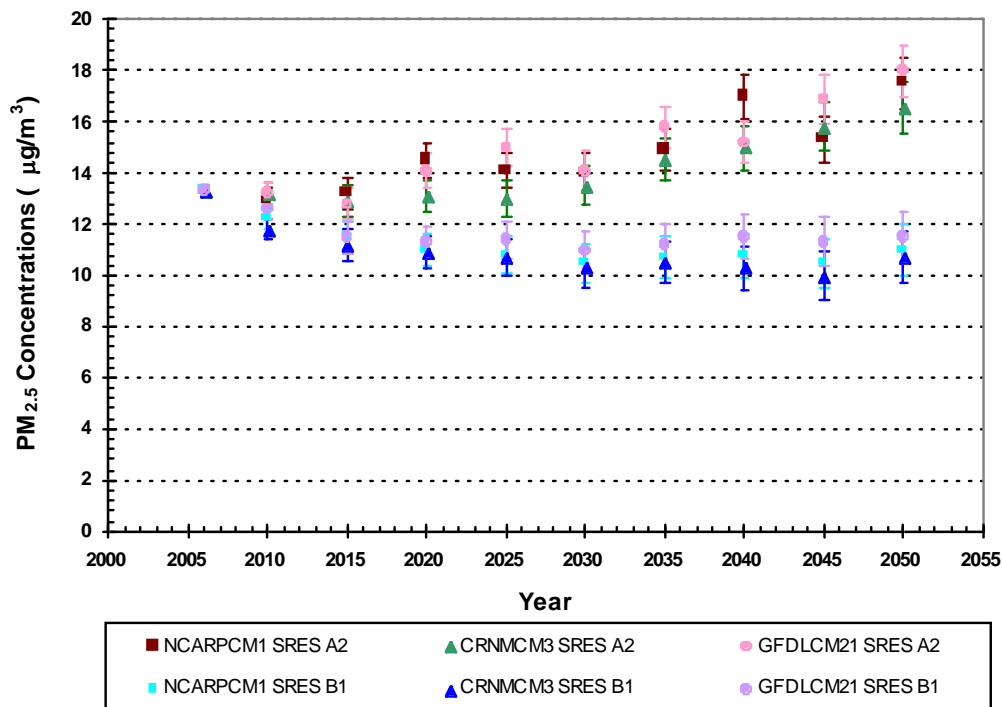
Figure 14. PM 2.5 projections
