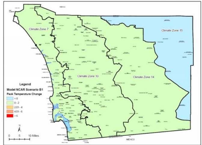
Change in Peak Temperatures by 2050 Model NCAR Scenario B1
