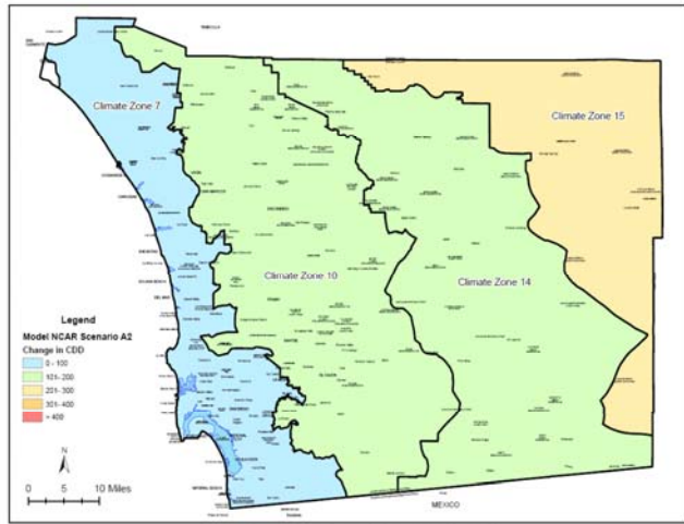
Change in Cooling Degree Days by 2050 Model NCAR Scenario A2
