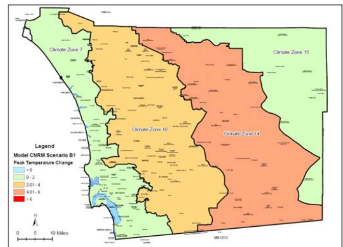
Change in Peak Temperatures by 2050 Model CNRM Scenario B1
