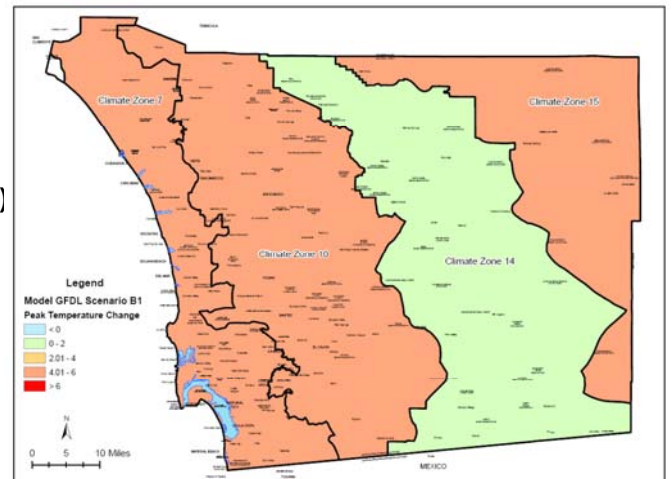
Change in Peak Temperatures by 2050 Model GFDL Scenario B1
