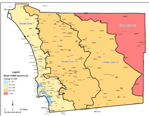
Change in Cooling Degree Days by 2050 Model CNRM Scenario A2
