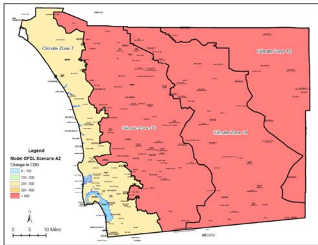
Change in Cooling Degree Days by 2050 Model GFDL Scenario A2
