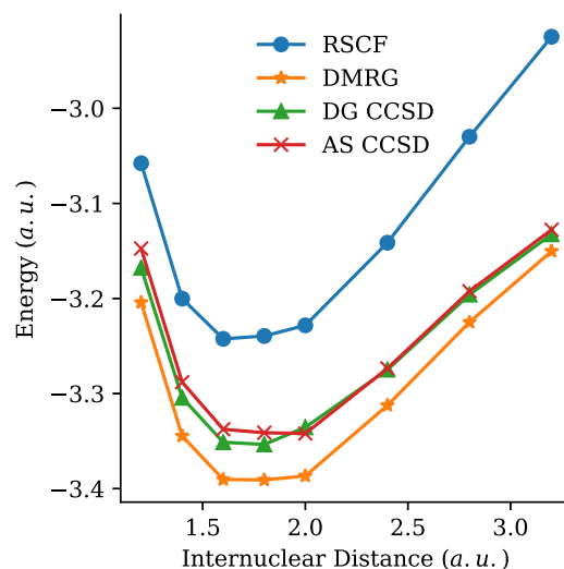
Figure C3. Potential energy surfaces for H_6 in a Gausset basis computed by restricted SCF, (DG-)CCSD and benchmarked with DMRG results. The averaged number of non-zero two-electron integrals per atom (DG-element \kappa ) is 287 762. The averaged number of non-zero two-electron integrals of the CAS calculations is 16 551.
