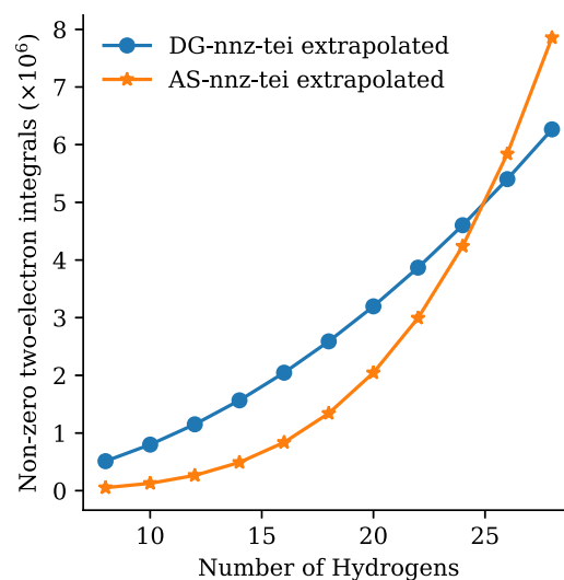
Figure C4. Extrapolation of non-zero two-electron integrals with 10 basis functions per DG element.
