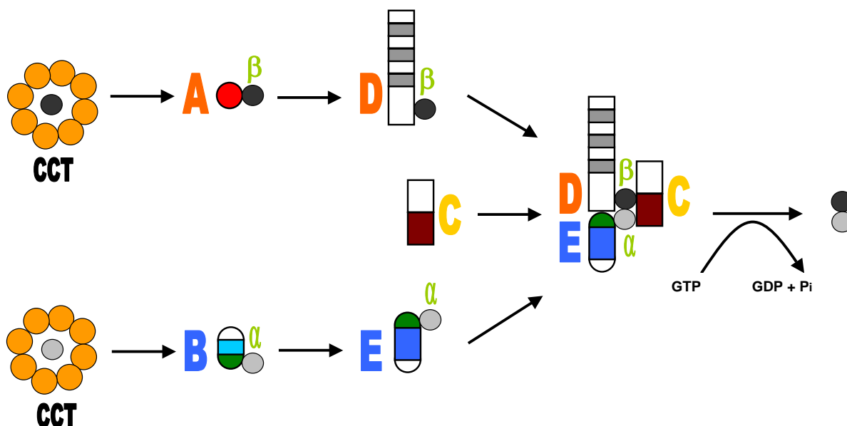
Figure 1 Simplified model depicting the reactions involved in the assembly of the tubulin heterodimer [18]. The colors depict the previously known regions of the cofactors and correspond to the colors ascribed to various domains in Figure 2A. The \alpha -tubulin is gray colored and \beta -tubulin is black colored. For clarity, the involvement of ADP ribosylation factor-like protein 2 (Arl2) in modulating the interaction of cofactors with tubulins [18] was omitted.
