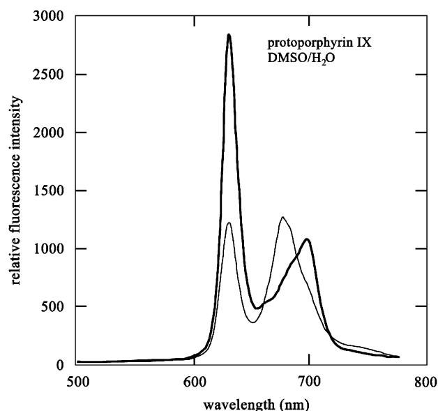
Fig. 3. The light exposure of a PP IX solution (solvent: DMSO and water) results in significant changes of the fluorescence spectrum due to the formation of fluorescent photoproducts (photoporphyrin) with an emission maximum at around 670 nm.
