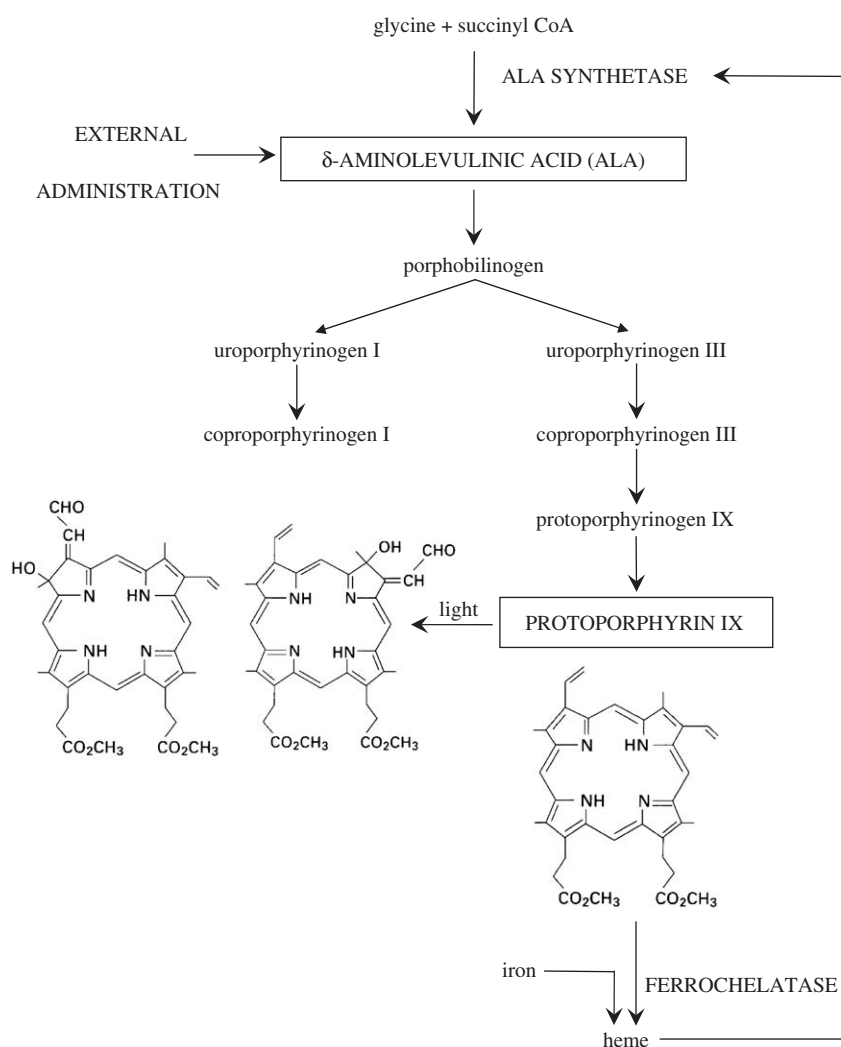
Fig. 1. Schematic pathway of stimulated biosynthesis of PP IX and its photodegradation. \delta -aminolevulinic acid synthase (ALAS) catalyzes within the mitochondria the condensation reaction between glycine and succinyl CoA and forms \delta -aminolevulinic acid (ALA). After synthesis of porphobilinogen, uro- and coproporphyrinogen, the photosensitive and fluorescent porphyrin PP IX is formed. PP IX is converted into the photostable non-fluorescent heme when iron as ferrous ion is inserted into the protoporphyrin ring by FECH activity. The concentration of heme regulates the activity of ALAS. The external application of ALA bypasses this regulation and results in an increased concentration of intracellular PP IX. Light activation of PP IX leads to desired photodynamic reactions as well as in its photodestruction by photobleaching and the formation of chlorin-type porphyrin isomers (photoprotoporphyrin) by single oxygen involved vinyl group oxidation and hydrogen rearrangement.
