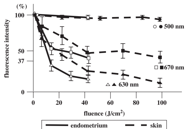
Fig. 5. Modification of fluorescence in endometrium and skin of PDT-treated living rats ( n = 6 ). No significant photoinduced changes of the natural occurring autofluorescence at around 500 nm occurred.
