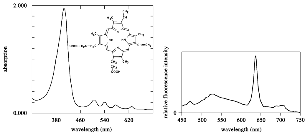
Fig. 2. Absorption spectrum of PP IX (left) and fluorescence spectrum of CHO cells 4 hours after incubation with ALA (right).
