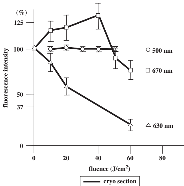
Fig. 6. Spectrally resolved fluorescence kinetics of 630 nm exposed cryosections ( n = 6 ).
