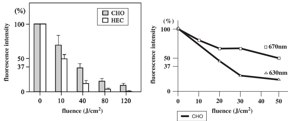
Fig. 4. Fluorescence modifications of ALA-incubated CHO and HEC cells due to 630 nm laser exposure. Left: results of flow cell cytometry showing the decay of the total fluorescence intensity in the red spectral range. Right: Typical spectrally resolved fluorescence modification in a single CHO cell demonstrating a different bleaching behavior at 630 nm (protoporphyrin) and 670 nm (protoporphyrin and photoporphyrin). In order to obtain corrected fluorescence values, the mean value of the fluorescence signal of control cells (no ALA) was subtracted from fluorescence values of ALA-sensitized cells.
