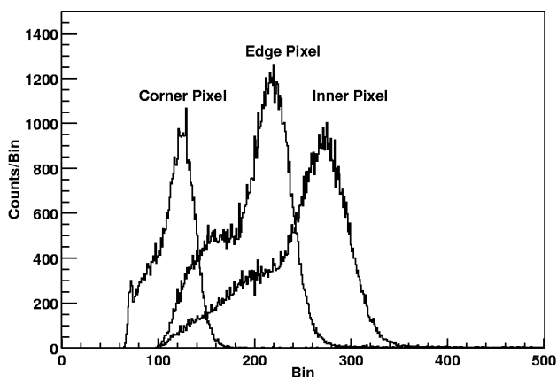
Fig. 6. Room temperature pulse height spectra for typical corner, edge and inner pixels excited by 140 keV emissions of ^{99\text{m}}\text{Tc} . The energy resolution of the corner, edge and inner pixels are 23.0%, 19.8% and 20.4% fwhm respectively
