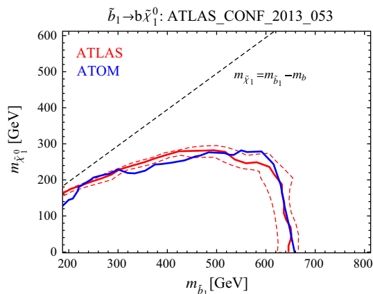
Fig. 38 The exclusion curves in the \tilde{b}_1 - \tilde{\chi}_1^0 simplified model parameter space ( \tilde{b}_1 \rightarrow b \tilde{\chi}_1^0 ). The red and blue curves are for ATLAS and ATOM, respectively. The red dashed curves show the 1-\sigma error band of the ATLAS exclusion curve
