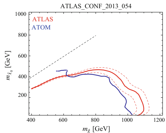
Fig. 39 The exclusion curves in the \tilde{g} - \tilde{\chi}_1^\pm - \tilde{\chi}_1^0 simplified model parameter space ( \tilde{g} \rightarrow qq \tilde{\chi}_1^\pm \tilde{\chi}_1^0 ). The chargino mass fixed at (m_{\tilde{g}} - m_{\tilde{\chi}_1^0})/2 . The red and blue curves are for ATLAS and ATOM, respectively. The red dashed curves show the 1-\sigma error band of the ATLAS exclusion curve
