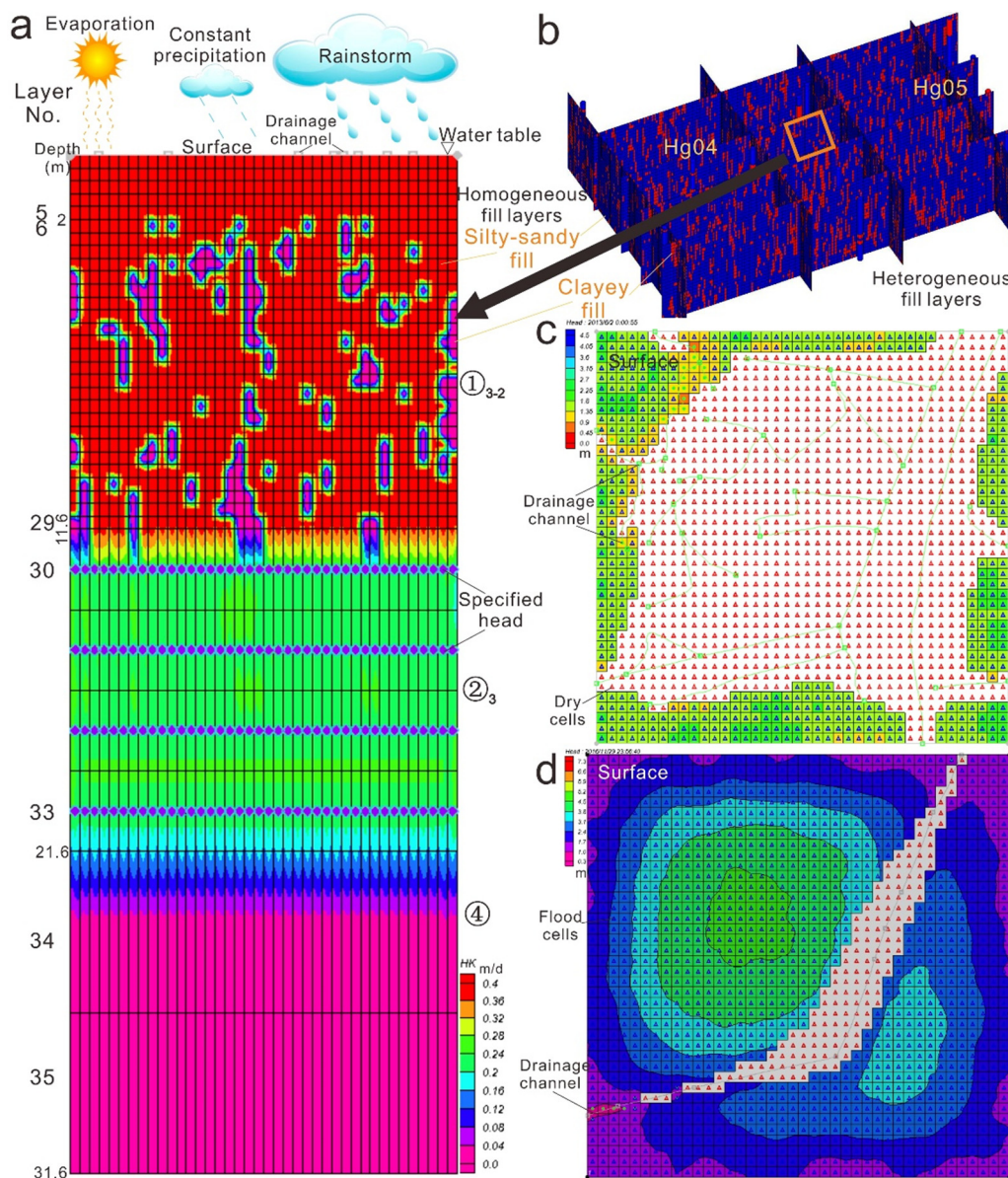
Fig. 2. Geo-model for the numerical analysis. a. K_p contour profile of comprehensive geo-model for the Zn transport modeling; b. Stochastic model for the heterogeneous reclaimed layers; c. Water head contour distribution in the surface layer after one year considering all the drainage channels; d. Water head contour distribution in the surface layer after over four year considering only one typical drainage channel.
