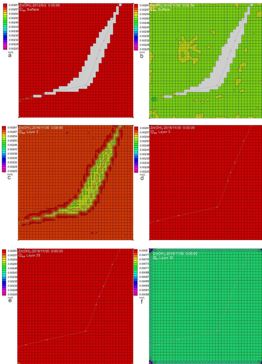
Fig. 7. Zn(OH)_2 concentration distribution within layers. a. Initial Zn(OH)_2 concentration distribution within surface on June 2nd 2012; b. Zn(OH)_2 concentration distribution within surface on November 30th 2016; c. Zn(OH)_2 concentration distribution within depth of 0.4–0.8 m on November 30th 2016; d. Zn(OH)_2 concentration distribution within bottom of heterogeneous fill (depth of 11.2–11.6 m) on November 30th 2016; e. Zn(OH)_2 concentration distribution within bottom of heterogeneous fill (depth of 11.2–11.6 m) on November 30th 2016; f. Zn(OH)_2 concentration distribution within top of stratum @_3 on November 30th 2016.
