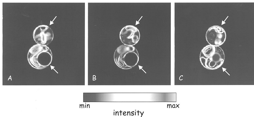
Fig. 2. Two-photon excitation LAURDAN fluorescence intensity images (false color representation) showing the movement of the internal structure of giant DLPC vesicles. Time zero image (A), after 2 (B) and 5 min (C). The temperature was 22°C. Frame size is 32 \times 32 \mu\text{m} .
