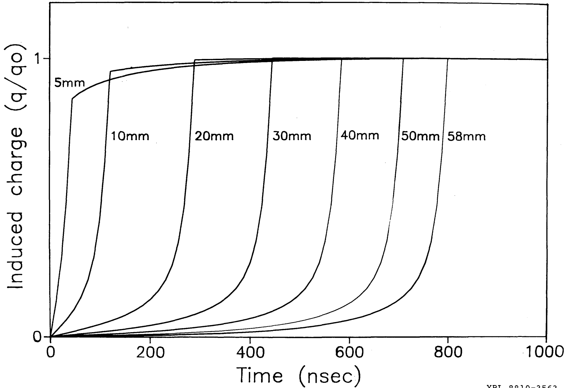
Fig. 7. Calculated pulse shapes due to point interactions along the detector axis at various distances from the n^+ electrode.
