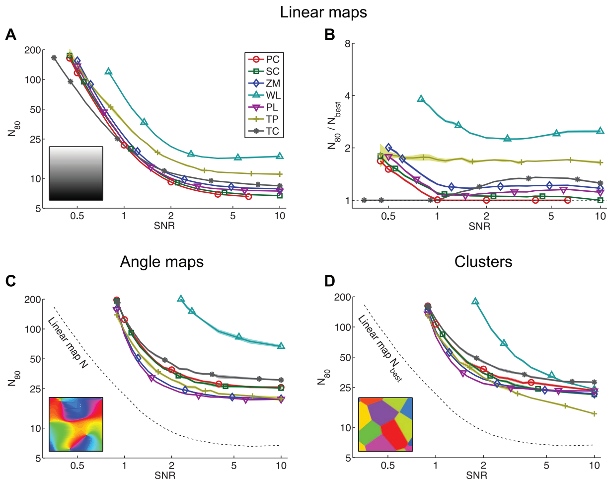
Figure 5. Comparison of the statistical power of seven map measures (PC: Pearson distance correlation, SC: Spearman distance correlation, ZM: Zehren measure, WL: wiring length, PL: path length, TP: topographic product, TC: topological correlation) when detecting (A) linear maps, (C) angle maps and (D) clusters. Power is summarized by the quantity N_{80} , the mean number of points (e.g. neurons, voxels) required to achieve a statistical power of 80%; this is shown as a function of the SNR. Panel B shows the relative powers of the measures for linear map detection; here N_{80} is normalized by N_{best} , the N_{80} of the most powerful measure for a given map type and SNR. For the angle maps and clusters the scale parameter s=0.4 and the insets show examples of the corresponding map type and scale. All axes have logarithmic scales. Missing data indicate that N_{80} is outside the range 7 \leq N \leq 200 . Uncertainty is depicted by shaded regions of \pm 1 StdErr. doi:10.1371/journal.pone.0087178.g005
