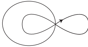
FIGURE 2.2. A cell graph of type (0, 1) with a vertex of degree 6.
