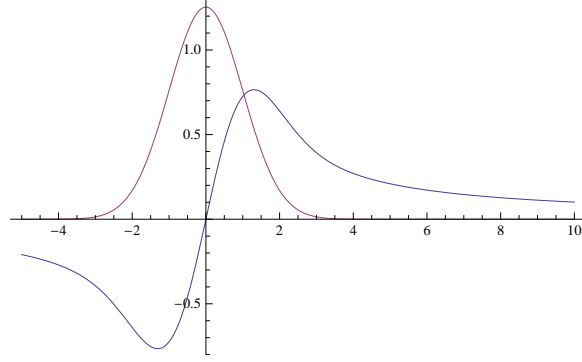
FIGURE 3.2. The imaginary part and the real part of \Psi^{\text{Catalan}}(x, 1) . For x \gg 0 , the imaginary part dies down, and only the real part has a non-trivial asymptotic expansion. Thus (3.51) is a series with real coefficients.
