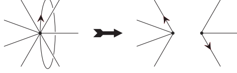
FIGURE 2.4. The process of contracting the arrowed loop E that is attached to p_1 .
