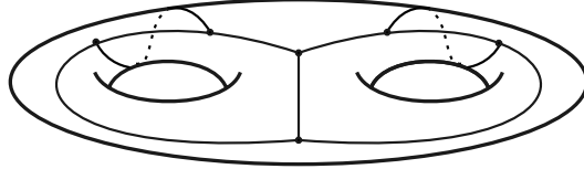
FIGURE 2.1. A cell graph of type (2, 6) .
