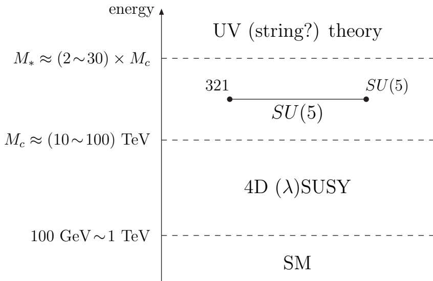
Figure 1: The schematic picture of our minimal theory. The standard model (SM) is the effective theory up to a scale of 100 \text{ GeV} \sim 1 \text{ TeV} , where it is replaced by a 4D (\lambda) SUSY model: a 4D N = 1 supersymmetric standard model with the superpotential given by Eq. (11) (in the minimal case). This model is further replaced at M_c \approx (10 \sim 100) \text{ TeV} by the minimal 5D SU(5) theory described in the text, which is the effective theory for the next factor of (2 \sim 30) . Finally, at the scale M_* \approx (2 \sim 30) \times M_c , the theory is embedded into a fundamental ultraviolet (UV) theory, which may be string theory.
