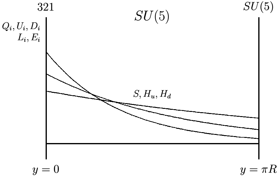
Figure 2: The schematic picture of the minimal model described in the text. The quark and lepton supermultiplets are localized (strongly) to the y = 0 brane. The wavefunction profiles for the S and Higgs fields are depicted arbitrarily.
