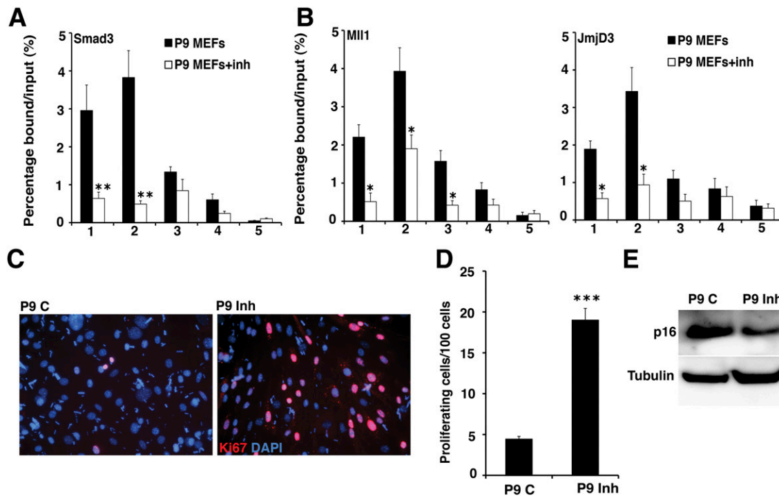
Figure 2—A: ChIP analysis comparing the recruitment of Smad3 to the Ink4a/Arf locus, in P9 MEFs in the presence (MEFs+inh) or absence of TGF- \beta inhibitor ( n = 3 ). 1–5 indicate the amplified regions, with 5 being the negative control. B: ChIP analyses comparing the recruitment of Mll1 and Jmjd3 to the Ink4a/Arf locus, in P9 MEFs treated with TGF- \beta inhibitor (MEFs+inh) or vehicle control ( n = 3 ). 1–5 indicate the amplified regions, with 5 being the negative control. Immunofluorescence (C) and quantification (D) for proliferation in P9 MEFs treated with TGF- \beta inhibitor (Inh) or vehicle control (C), using immunostaining with Ki67 antibody (red), counterstained with DAPI (blue) to mark the nuclei ( n = 3 ). E: Western blotting for p16 and \beta -tubulin in cell extracts from P9 MEFs treated with TGF- \beta inhibitor (Inh) or vehicle control (C). Representative experiment from n = 3 . Error bars indicate \pm SEM. P values were determined by unpaired Student t test. * P < 0.05 ; ** P < 0.01 ; *** P < 0.001 .
