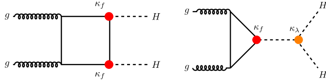
Fig. 1. Feynman diagrams for the LO HH production via gluon fusion. \kappa_f corresponds to the modifier of the Higgs boson coupling strength (Section 4) to fermions.
