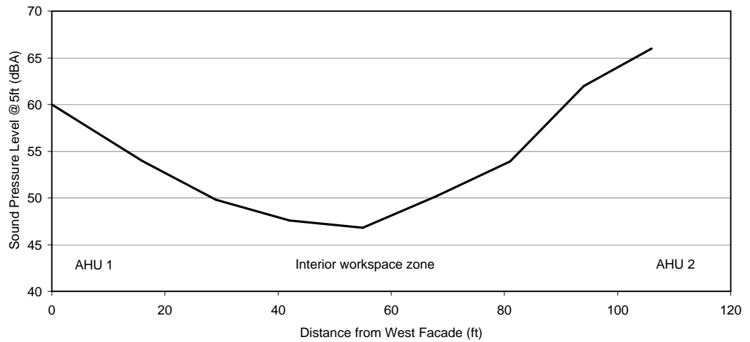
Figure 4.8 Ambient sound level readings
