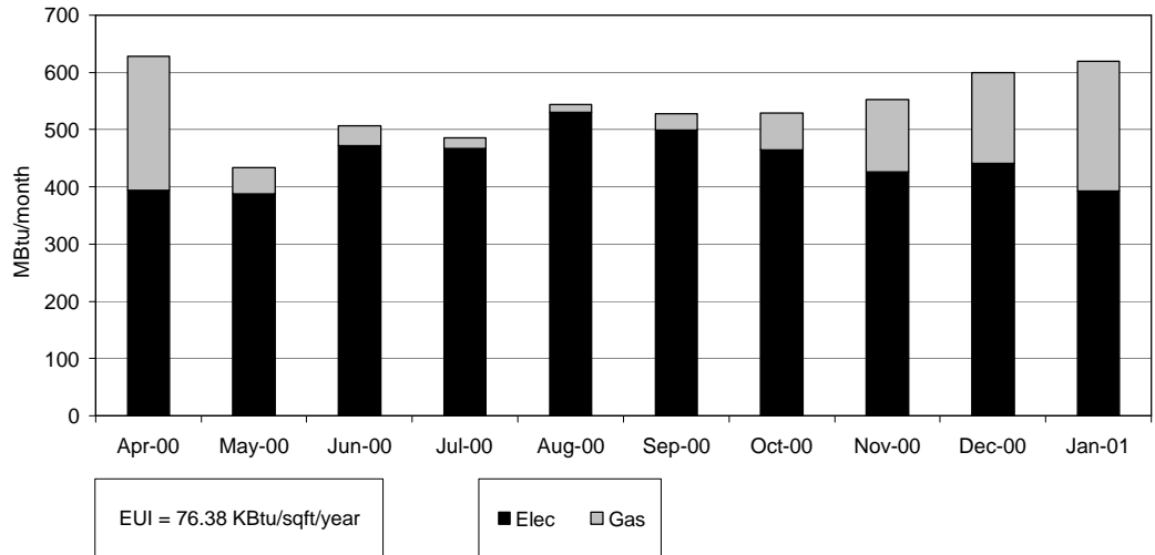
Figure 4.7 Monthly energy use
