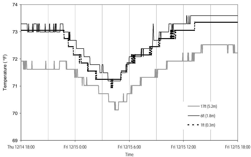
Figure 4.3 Weekday interior room air temperatures over a 24-hour period
