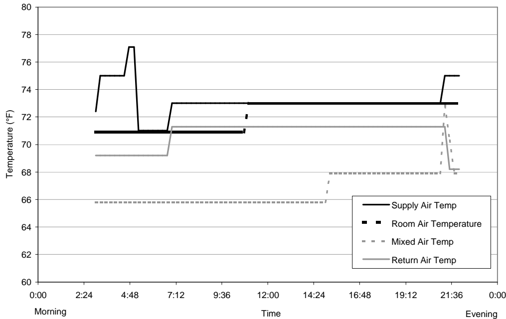
Figure 4.1 Temperature profiles under winter day operation
