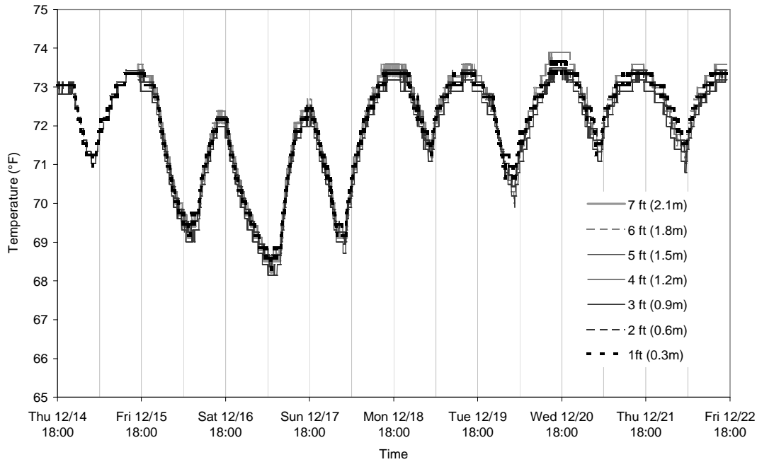
Figure 4.2 Typical weekly internal zone room air temperatures
